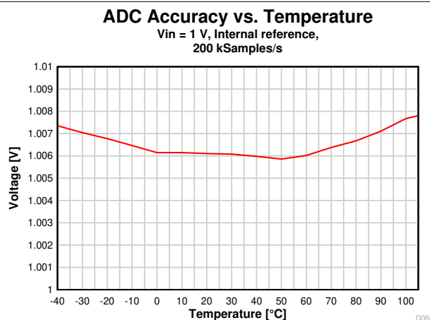
Figure 7-37. ADC Accuracy vs. Temperature
