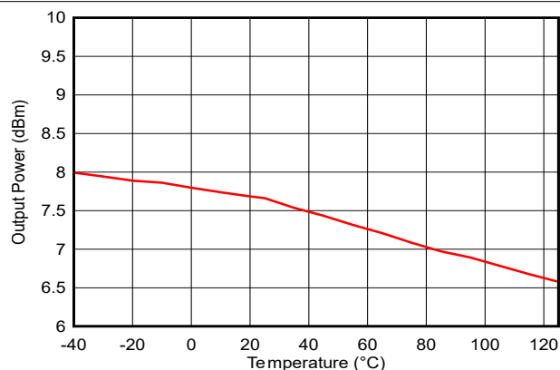
Figure 7-22. Output Power vs. Temperature (Bluetooth LE 1Mbps, 2.44GHz, +8dBm)
