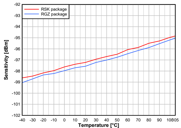
Figure 7-19. Sensitivity vs. Temperature (BLE 1 Mbps, 2.44GHz)
