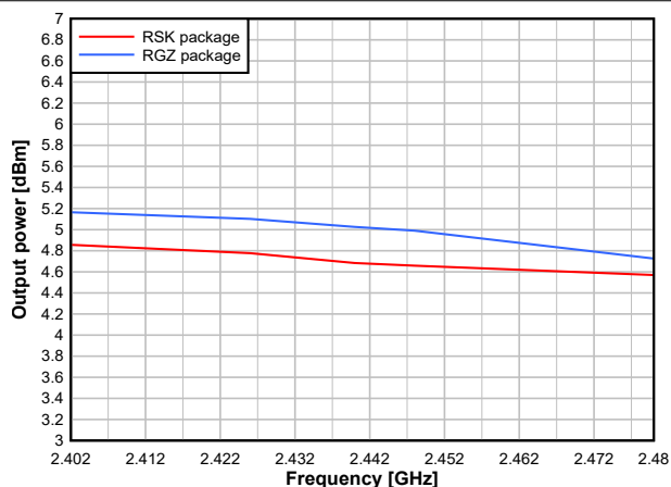
Figure 7-34. Output Power vs. Frequency (BLE 1Mbps, 2.44GHz, +5dBm)
