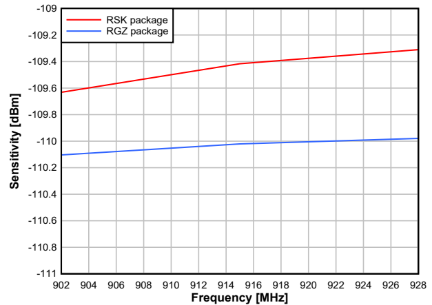
Figure 7-15. Sensitivity vs. Frequency (50kbps, 915MHz)
