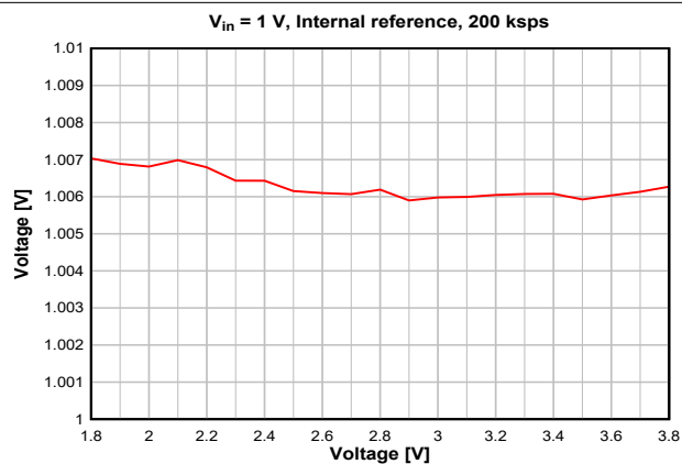
Figure 8-40. ADC Accuracy vs. Supply Voltage (VDD)
