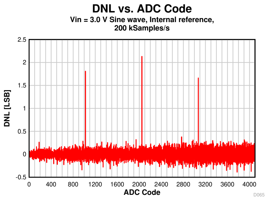
Figure 8-46. DNL vs. ADC Code
