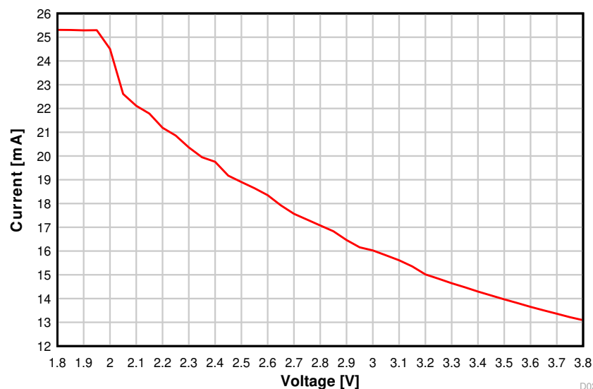
Figure 8-15. TX Current vs. Supply Voltage (VDDS) (50 kbps, 868.3 MHz)
