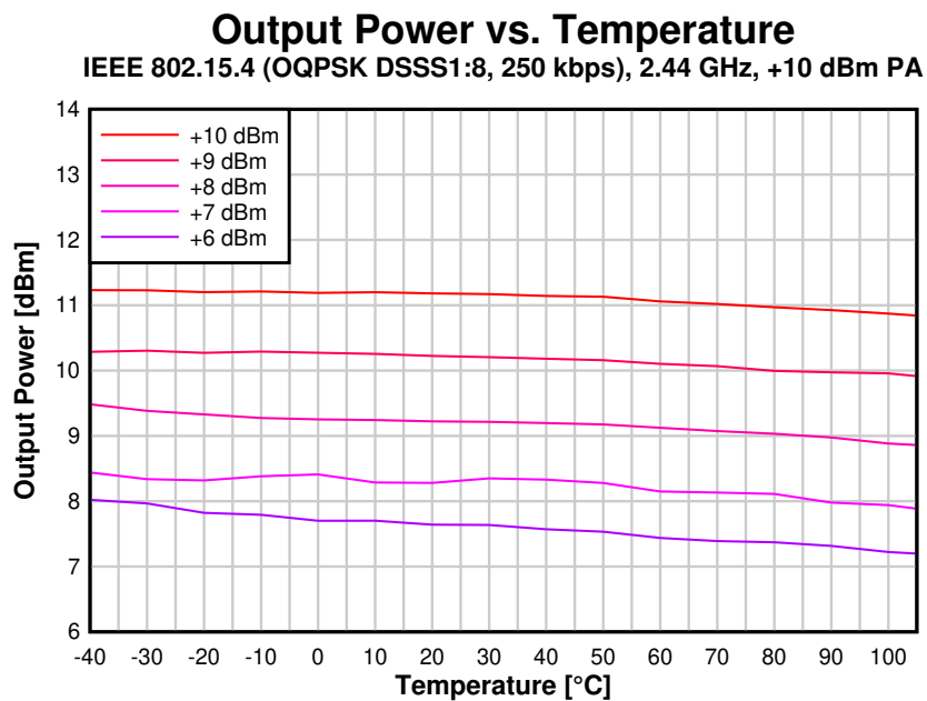
Figure 8-44. Output Power vs. Temperature (2.44 GHz, +10 dBm PA)
