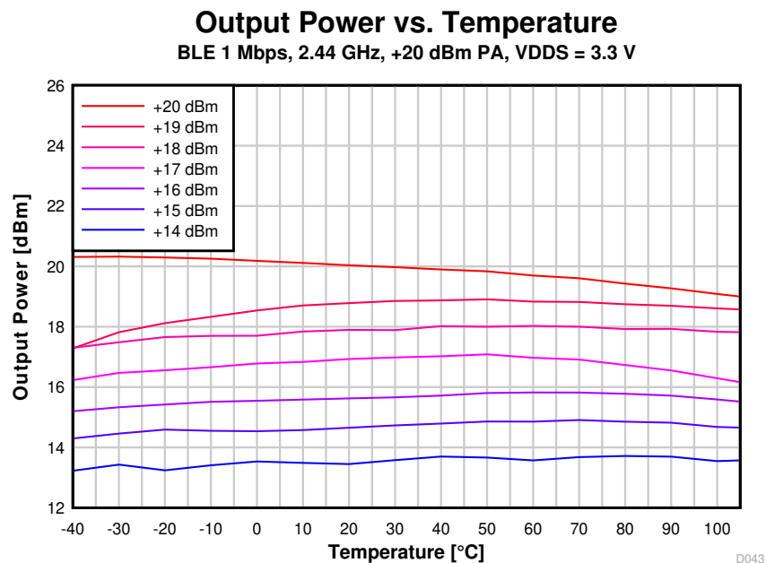
Figure 8-43. Output Power vs. Temperature (BLE 1 Mbps, 2.44 GHz, +20 dBm PA)
