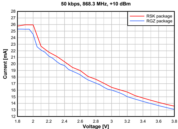
Figure 7-9. TX Current vs. Supply Voltage (VDDSD) (50kbps, 868.3MHz)
