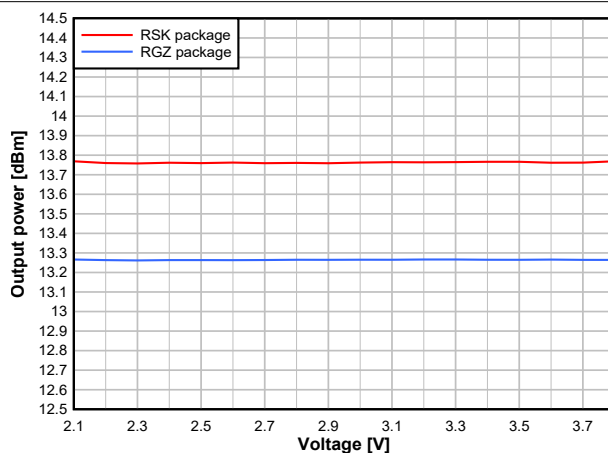
Figure 7-16. Output Power vs. Supply Voltage (VDDS) (50kbps, 868.3MHz, +14dBm)
