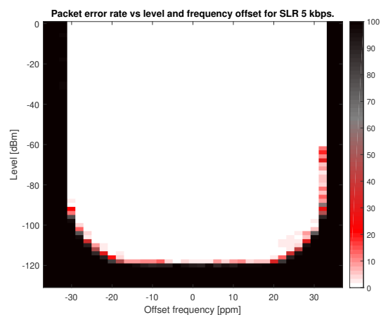
Figure 7-15. PER vs. Level vs. Frequency (SimpleLink™ Long Range 5 kbps, 868 MHz)
