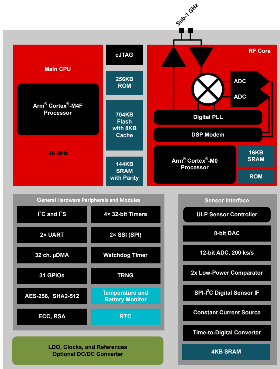
Figure 3-1. CC1312R7 Block Diagram
