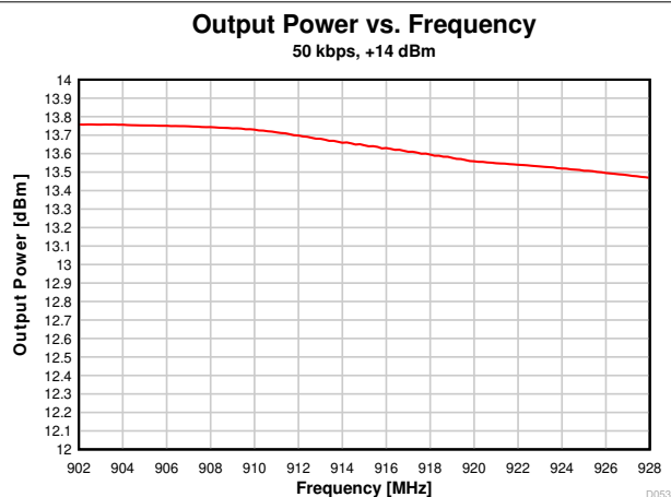
Figure 7-21. Output Power vs. Frequency (50 kbps, 915 MHz)
