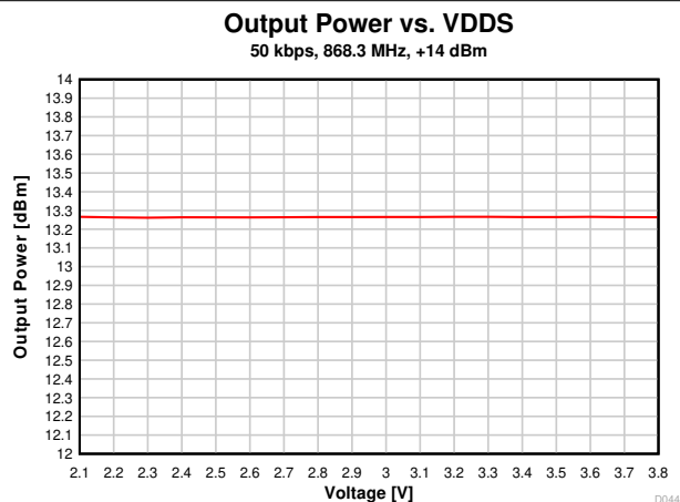
Figure 7-19. Output Power vs. Supply Voltage (VDD5) (50 kbps, 868.3 MHz)
