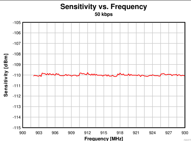
Figure 7-11. Sensitivity vs. Frequency (50 kbps, 915 MHz)
