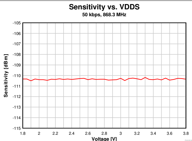
Figure 7-13. Sensitivity vs. Supply Voltage (VDD) (50 kbps, 868.3 MHz)
