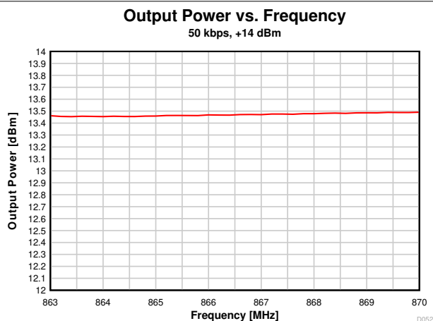
Figure 7-20. Output Power vs. Frequency (50 kbps, 868 MHz)
