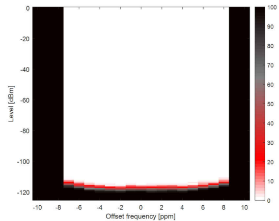
Figure 7-17. Narrowband, 9.6 kbps \pm 2.4 kHz deviation, 2-GFSK, 868 MHz, 17.1 kHz RX Bandwidth
