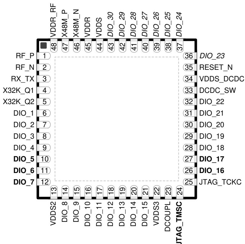
Figure 6-1. RGZ (7-mm x 7-mm) Pinout, 0.5-mm Pitch (Top View)
