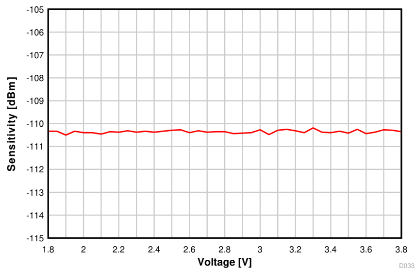
Figure 8-15. Sensitivity vs. Supply Voltage (VDDIS) (50 kbps, 868.3 MHz)
