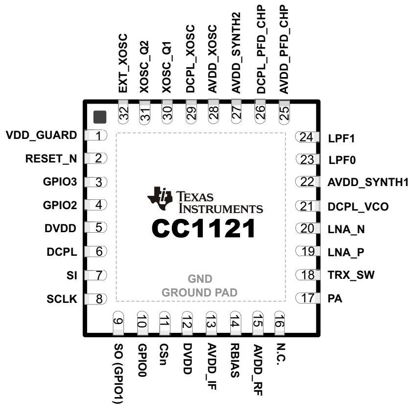
Figure 5-1. Package 5-mm × 5-mm QFN
