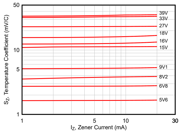
Figure 6-2. Temperature Coefficient
