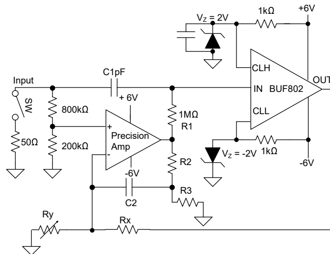
Figure 7-13. Composite Loop Using BF Mode
