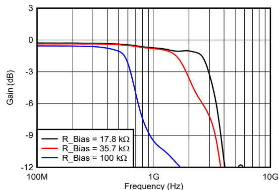
Figure 5-6. Frequency Response vs R_Bias Resistance
