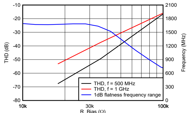
Figure 7-6. THD and Bandwidth vs R_{Bias}
