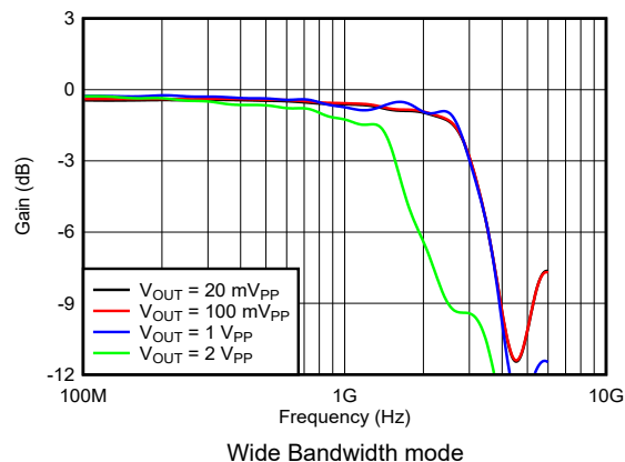
Figure 5-1. Frequency Response vs Output Voltage
