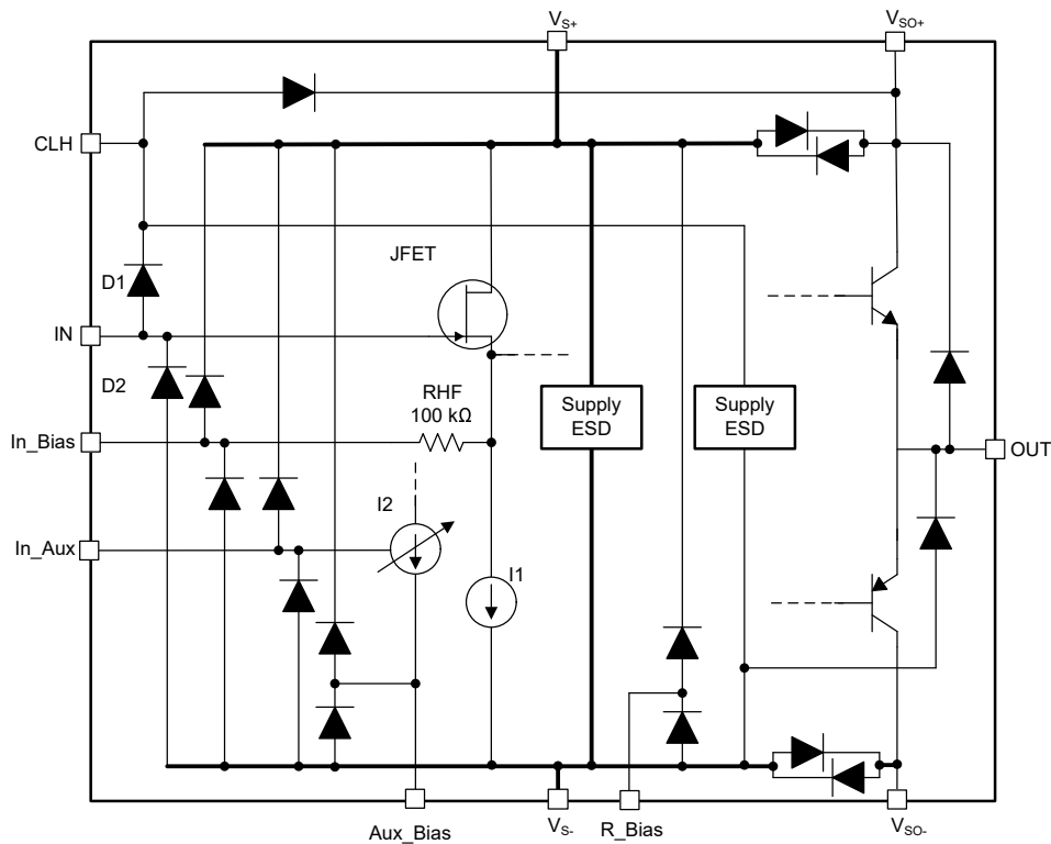
Figure 7-7. Internal ESD Structure
