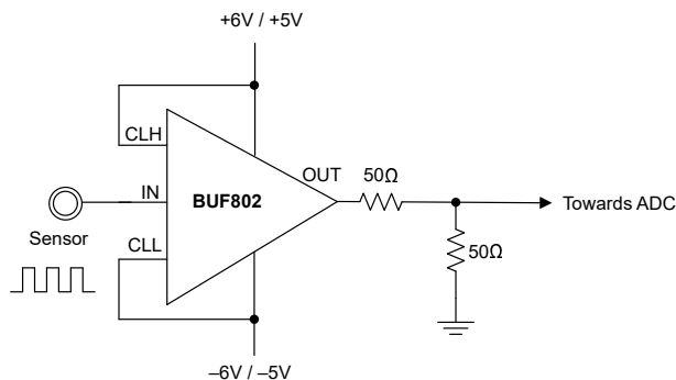
Figure 7-10. BUF802 DC Mode
