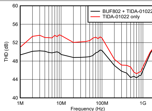
Figure 8-8. Total Harmonic Distortion (THD) vs Frequency
