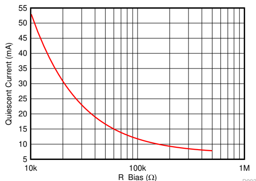
Figure 7-5. Quiescent Current vs R_{Bias}
