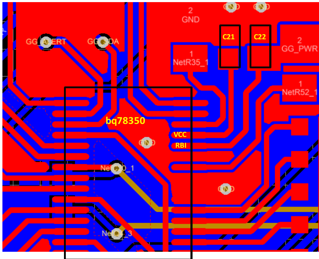
Figure 17. bq78350 Layout
