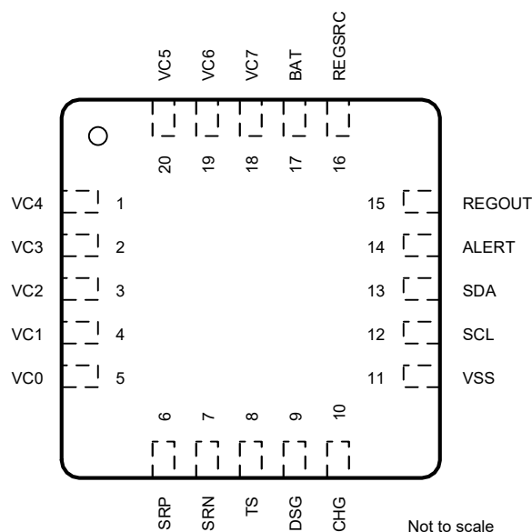
Figure 5-1. BQ77307 Pinout
