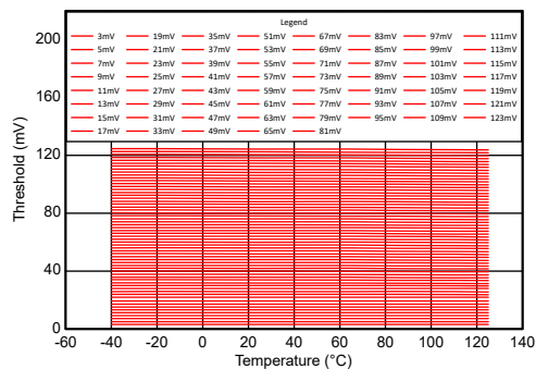
Figure 6-7. Overcurrent in Charge Protection (OCC) Threshold vs. Temperature
