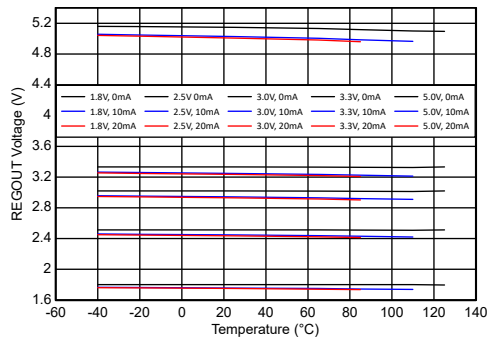
Figure 6-9. REGOUT Voltage vs. Temperature and Load
