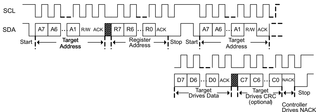
Figure 7-4. I²C Read Without Repeated Start
