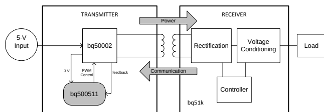
Simplified Schematic
