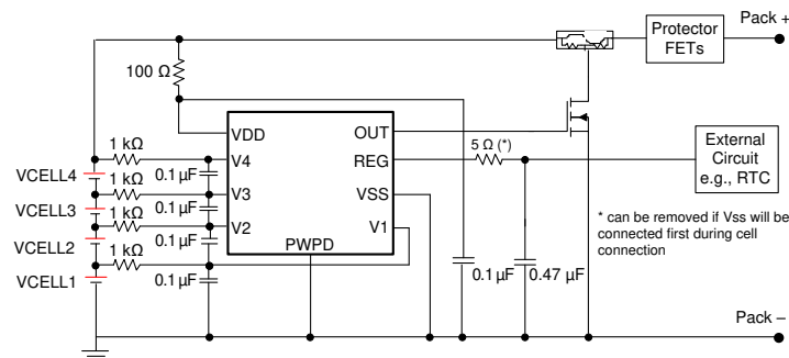
Simplified Schematic
