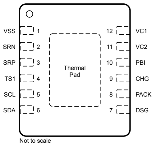
Figure 6-1. DRZ Package 12-Pin VSON Top View
