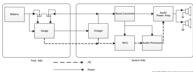
Wireless (Bluetooth®) Speaker Application Block Diagram
