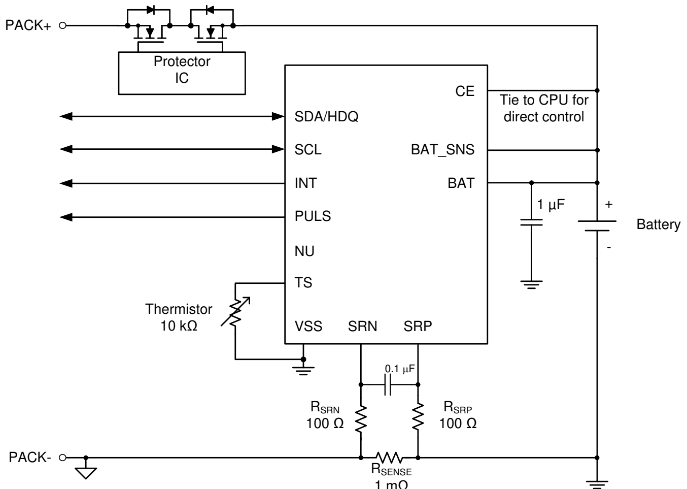
Figure 7-1. BQ27Z561 1-Series Cell Typical Implementation
