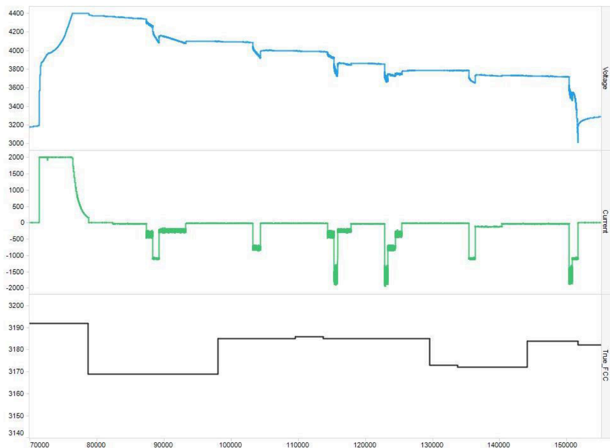
Figure 7-2. Full Charge Capacity Tracking (X-Axis Is Seconds)
