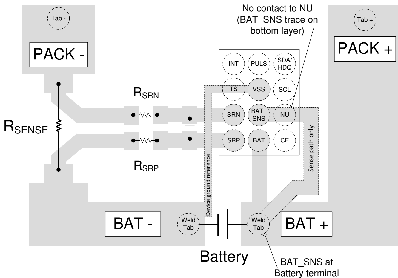
Figure 7-3. BQ27Z561 Key Trace Board Layout
