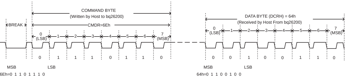
Figure 4. Communication Sequence
