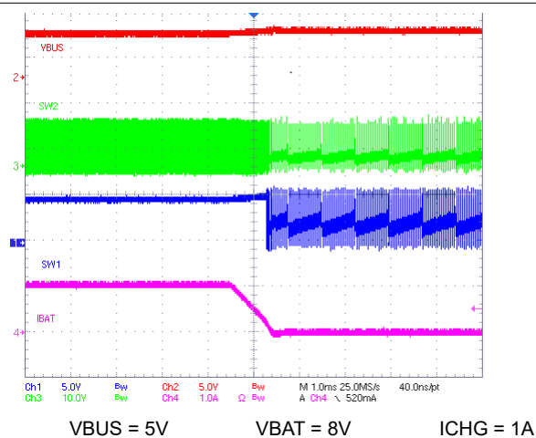
Figure 8-7. Charge Disable
