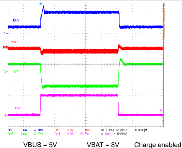
Figure 8-16. IINDPM Transient Response
