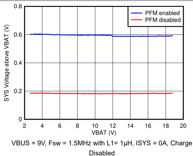
Figure 6-20. Offset Voltage of SYS Regulation above VBAT
