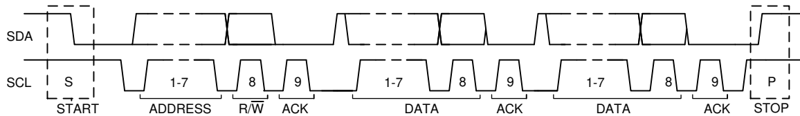
Figure 7-20. Complete Data Transfer on the I²C Bus
