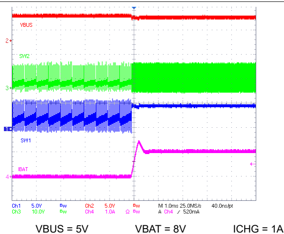
Figure 8-6. Charge Enable
