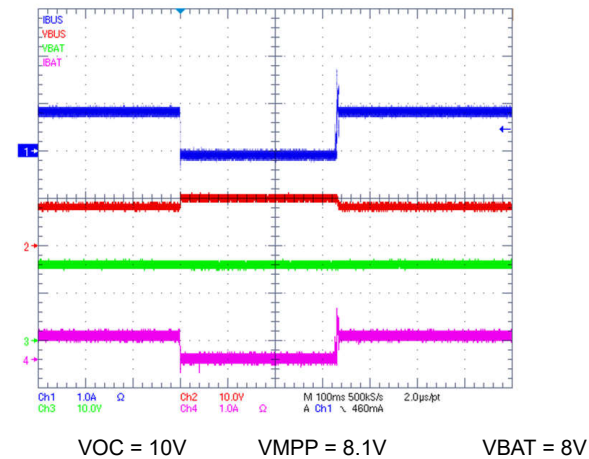
Figure 8-19. MPPT Operation Zoom
