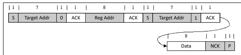
Figure 7-22. Single Read
