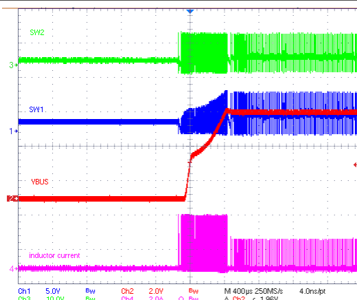
Figure 8-11. Buck Mode PFM with OOA
