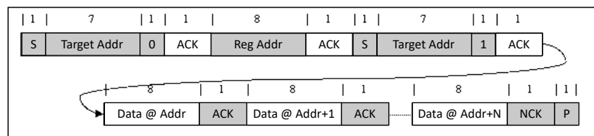
Figure 7-24. Multi-Read
