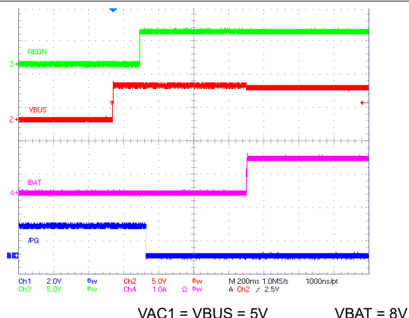
Figure 8-5. Power Up from VAC1 with Charge Enabled
