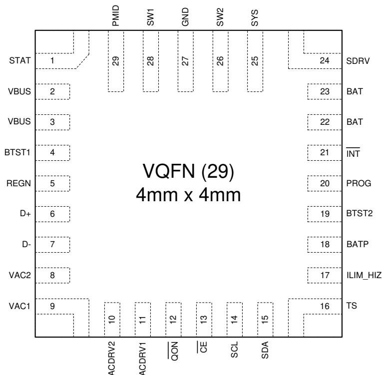
Figure 5-1. RQM Package, 29-Pin VQFN-HR (Top View)
