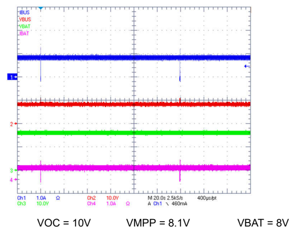
Figure 8-18. MPPT Operation
