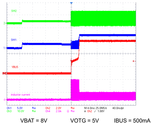
Figure 8-14. OTG Startup at 500-mA Load
