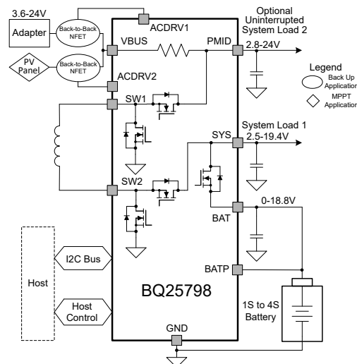
Simplified Schematic
