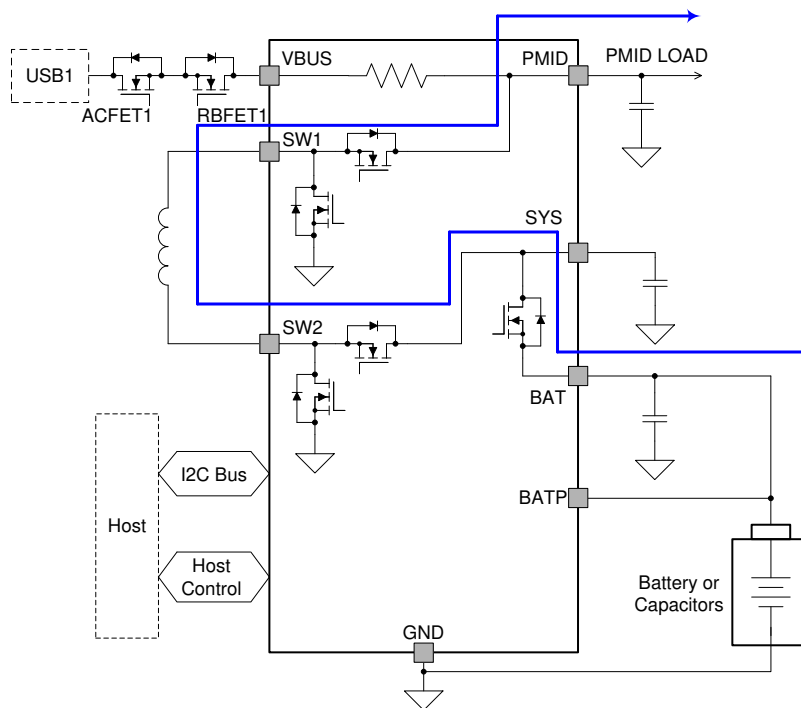
Figure 7-6. The Simplified Application Diagram for the Backup Mode
