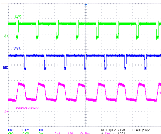
Figure 8-9. Buck-Boost Charging Mode PWM Operation
