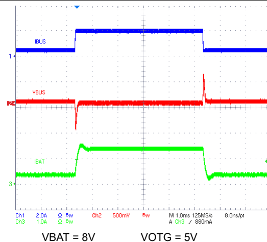
Figure 8-17. VOTG Load Transient Response
