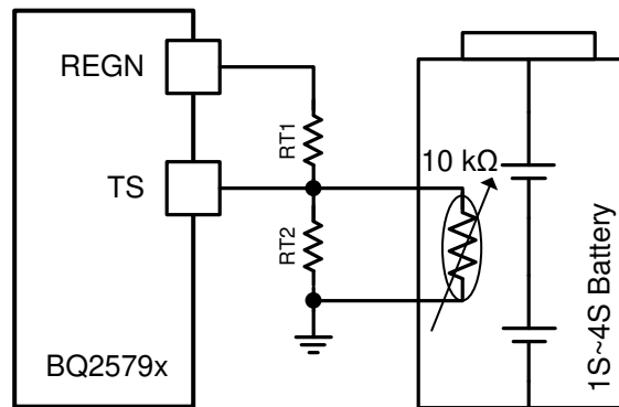
Figure 7-12. TS Resistor Network
