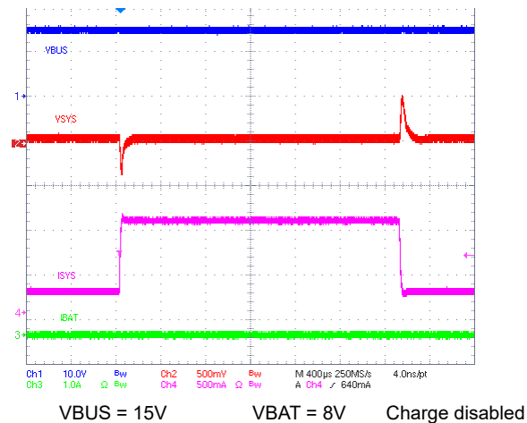
Figure 8-15. VSYS Load Transient Response
