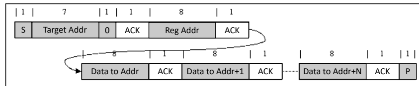
Figure 7-23. Multi-Write
