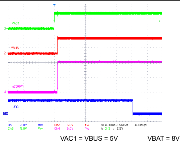
Figure 8-4. ACFET1-RBFET1 Turns on at Power Up
