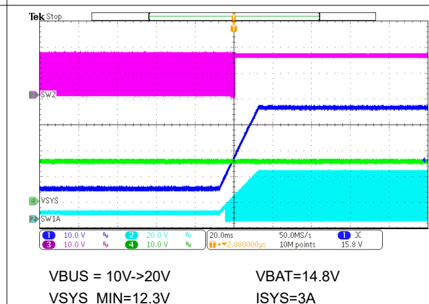
Figure 8-6. Line Regulation
