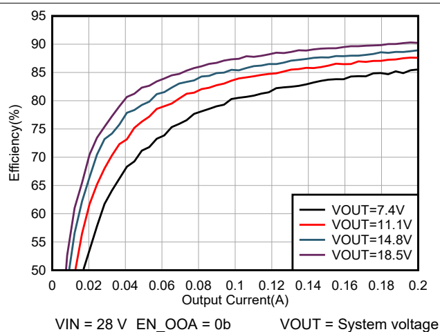
Figure 6-9. Light Load System Efficiency
