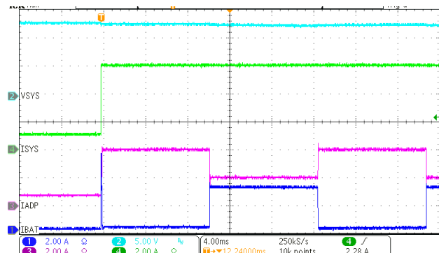
Figure 8-22. Automatic Second Phase Adding and Dropping Under 28-V VBUS
