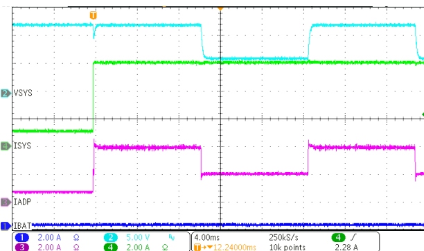
Figure 8-21. Automatic Second Phase Adding and Dropping Under 36-V VBUS
