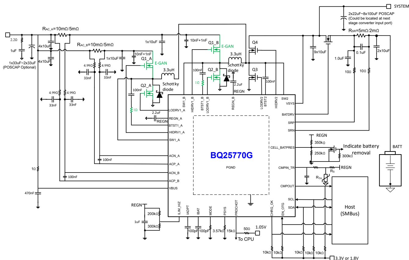
Figure 8-1. Application Diagram of BQ25770G
