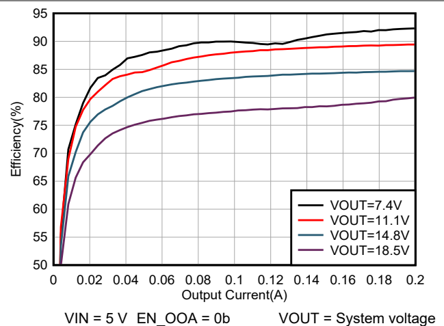
Figure 6-6. Light Load System Efficiency
