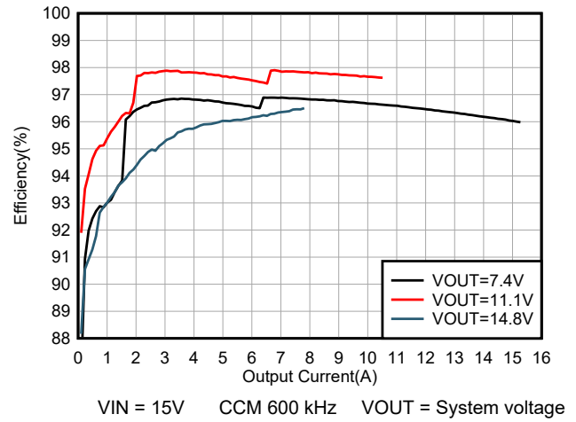
Figure 6-2. System Efficiency
