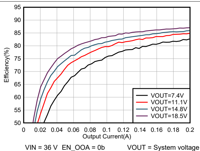
Figure 6-10. Light Load System Efficiency
