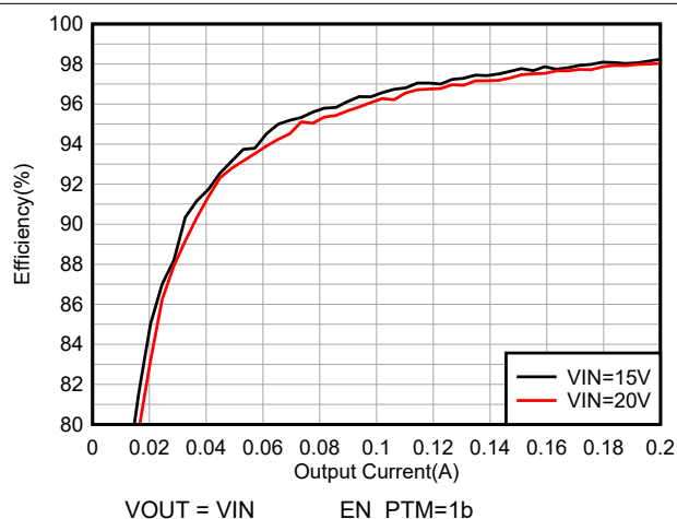
Figure 6-12. PTM Mode Light Load System Efficiency
