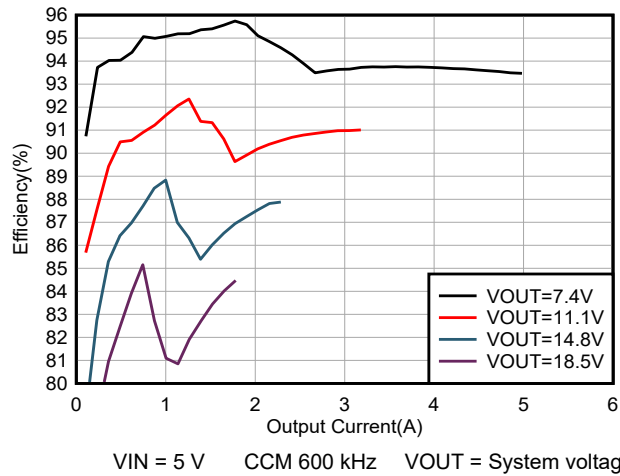
Figure 6-1. System Efficiency
