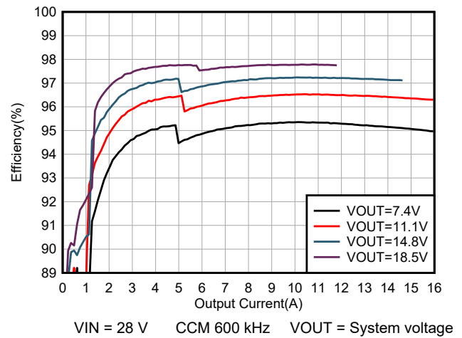
Figure 6-4. System Efficiency
