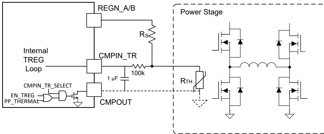
Figure 7-5. Recommended Configuration for CMPIN_TR Temperature Regulation
