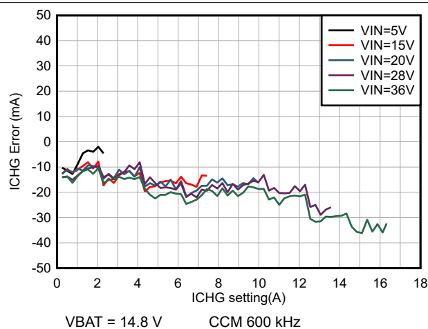
Figure 6-15. Battery Charge Current Regulation Accuracy
