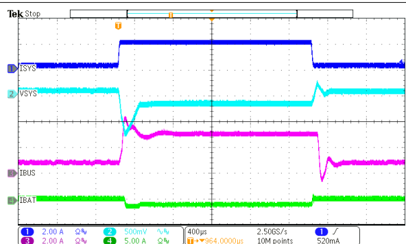
Figure 8-14. Input Current Regulation in Buck Mode
