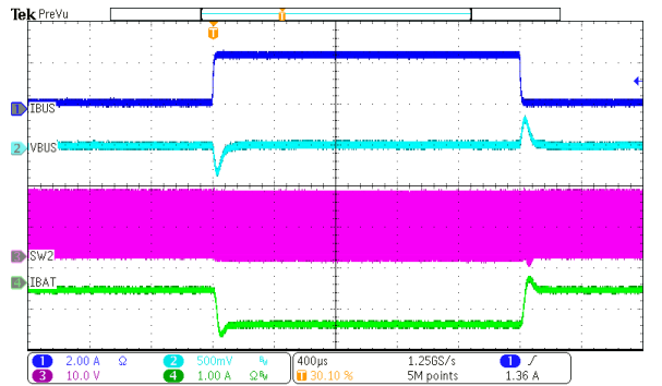
Figure 8-19. OTG Load Transient
