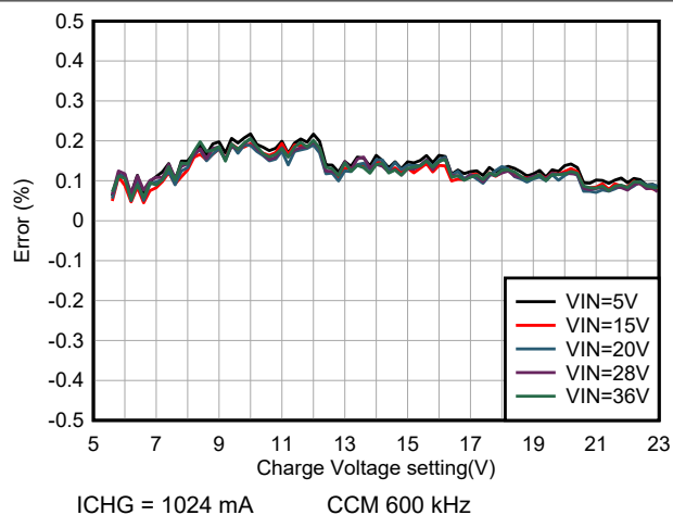
Figure 6-14. Battery Voltage Regulation Accuracy
