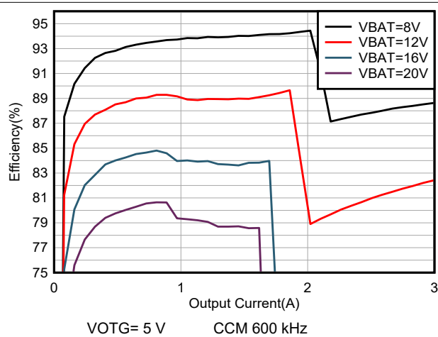
Figure 6-11. OTG Efficiency
