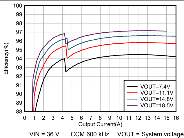
Figure 6-5. System Efficiency
