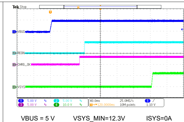
Figure 8-4. Power Up From 5 V
