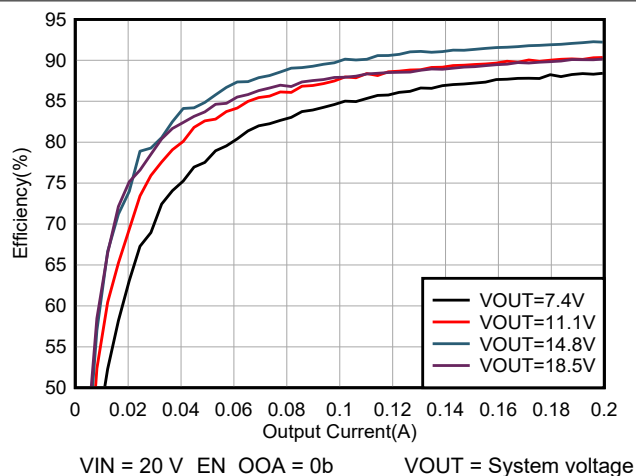
Figure 6-8. Light Load System Efficiency
