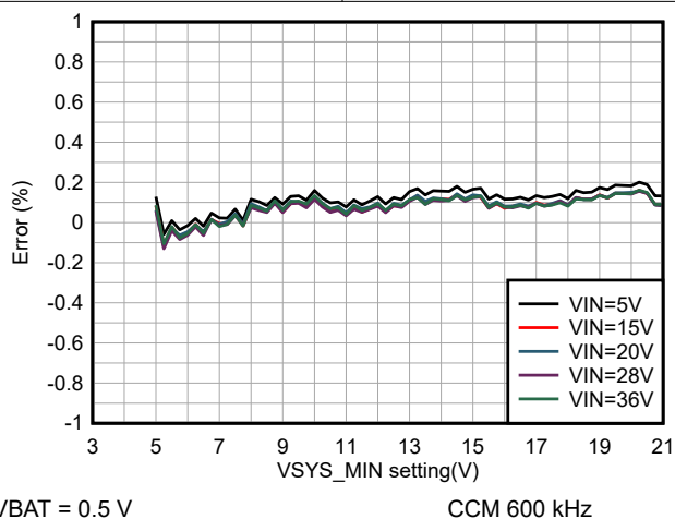
Figure 6-17. Minimum System Voltage Regulation Accuracy
