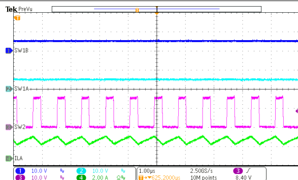
Figure 8-7. PFM Operation
