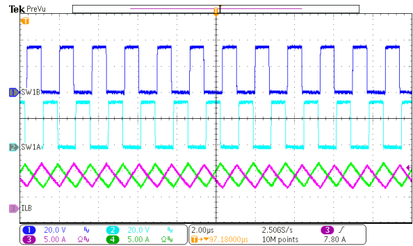
Figure 8-20. Dual Phase Current Balance at 36 V 180 W
