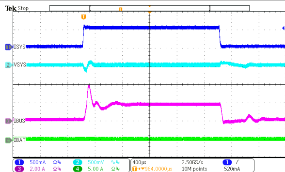
Figure 8-13. System Regulation in Boost Mode
