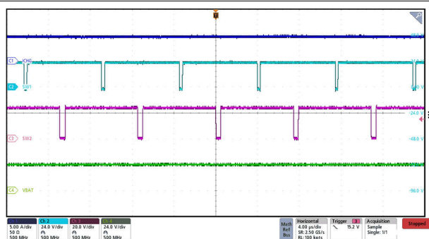
VAC = 24 V VBAT = 20 V ICHG = 5 A Figure 9-9. Buck Switching Waveform
