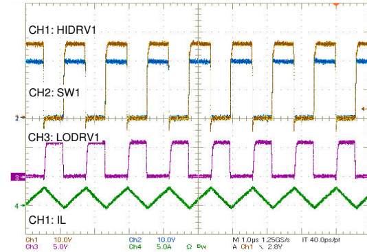
Figure 10-8. PWM Operation
