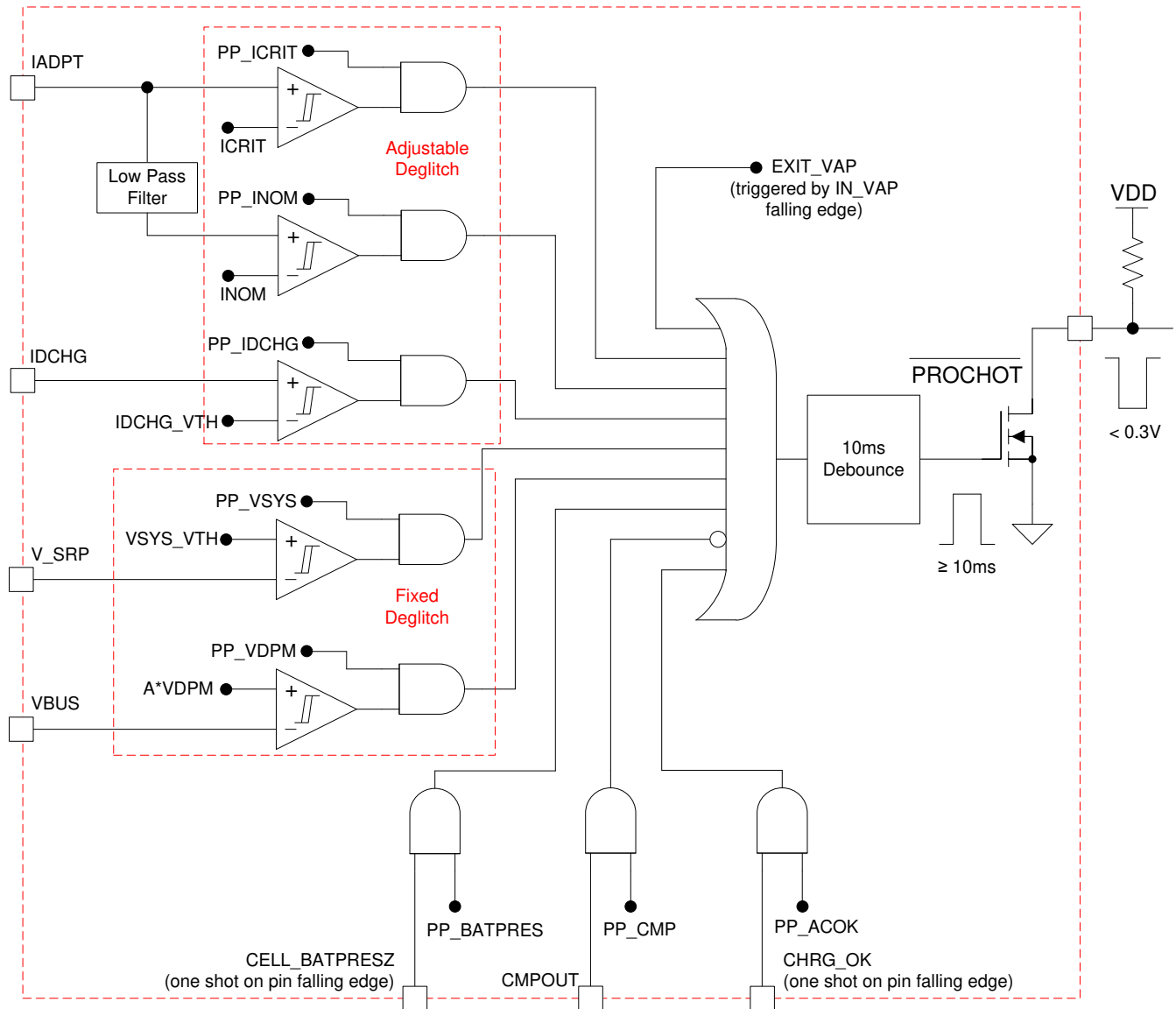
Figure 9-2. PROCHOT Profile
