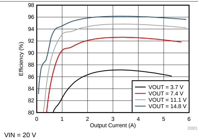
Figure 7. System Efficiency
