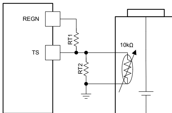
Figure 8-6. TS Resistor Network
