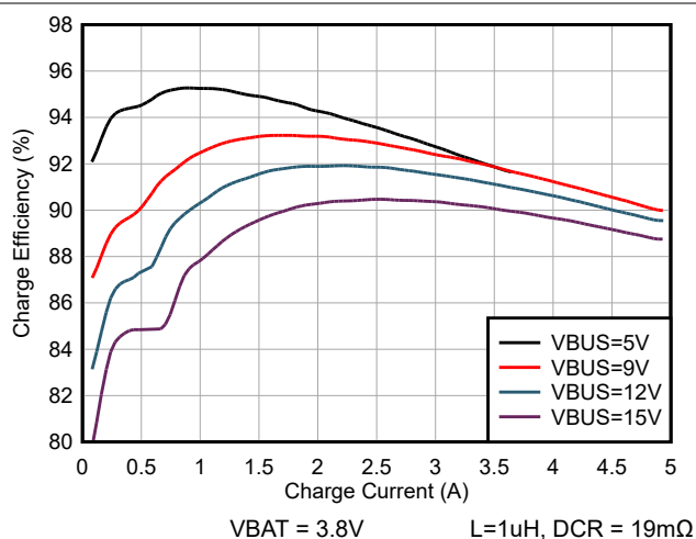
Figure 7-2. Charge Efficiency vs Charge Current
