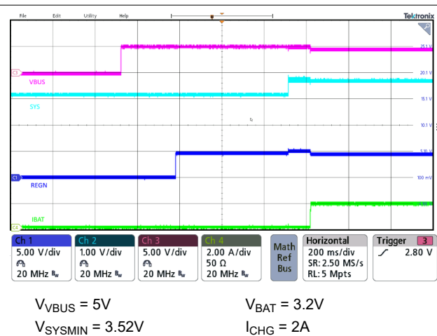
Figure 9-5. Power-Up Sequence
