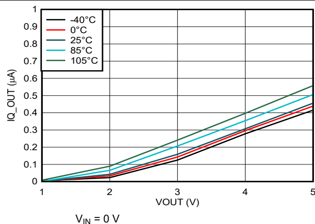
Figure 6-9. Output Quiescent Current vs Output Voltage
