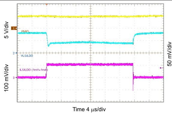
Figure 10-54. 1.8 V LSDO Load Transient, 0 to 100 mA
