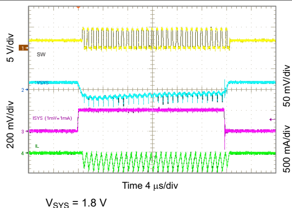
Figure 10-39. 1.8 V_{SYS} Load Transient, 0 to 200 mA
