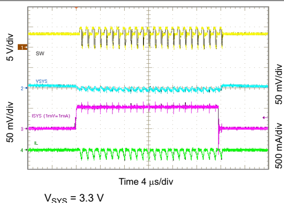
Figure 10-37. 3.3 V_{SYS} Load Transient, 0 to 50 mA
