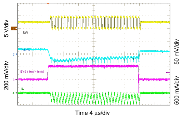
Figure 10-41. 2.5 V_{SYS} Load Transient, 0 to 200 mA
