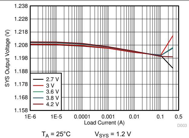
Figure 10-15. 1.2 V_{\text{SYS}} Load Regulation
