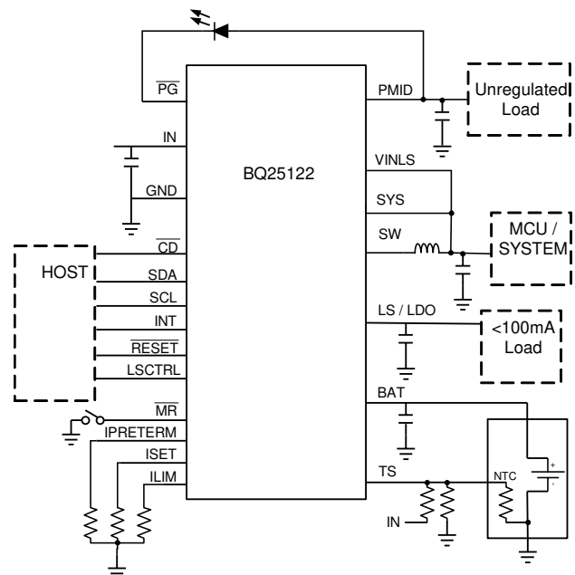
Simplified Schematic
