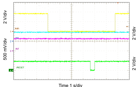
Figure 10-65. RESET Timing
