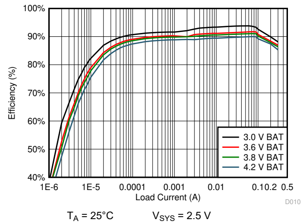
Figure 10-13. 2.5 V_{\text{SYS}} System Efficiency
