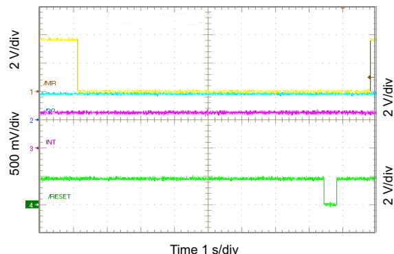
Figure 10-66. RESET Timing
