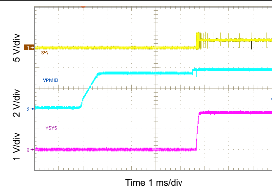
Figure 10-43. Startup Showing SS on SYS in PWM Mode
