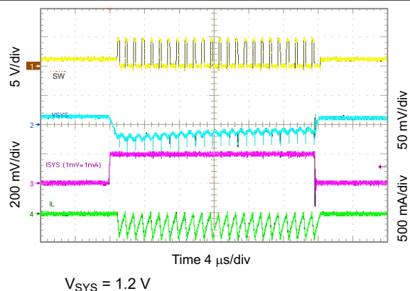
Figure 10-38. 1.2 V_{SYS} Load Transient, 0 to 200 mA
