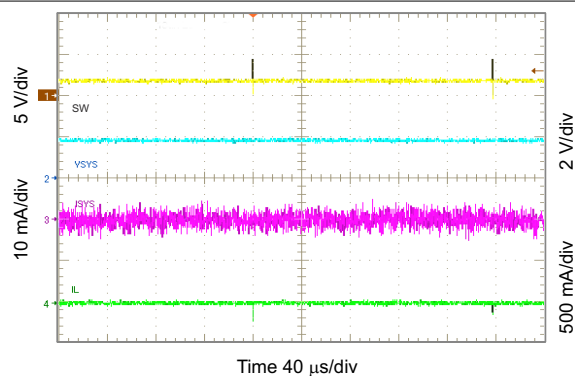
Figure 10-24. 3.3 V_{\text{SYS}} Line Regulation
