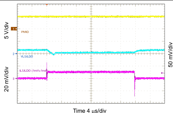
Figure 10-49. 1.8 V LSLDO Load Transient, 0 to 10 mA
