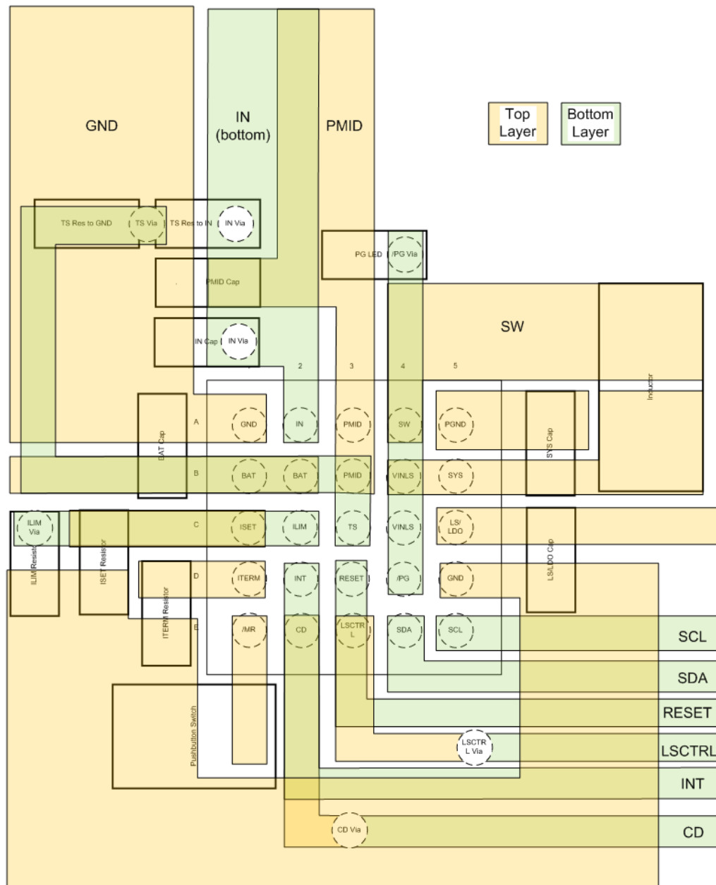
Figure 12-1. BQ25122 Layout
