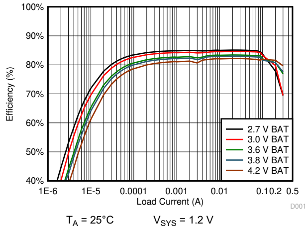
Figure 10-10. 1.2 V_{\text{SYS}} System Efficiency
