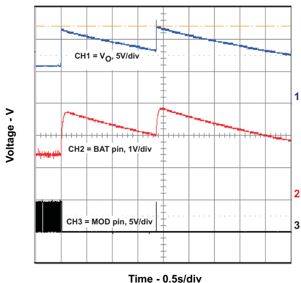
Figure 13. Battery Removal During Fast Charge
