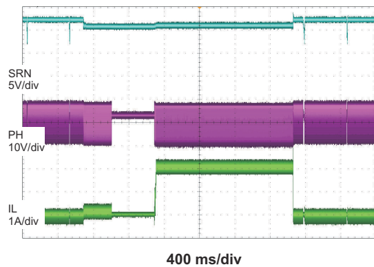
Figure 8-9. Battery Insertion and Removal
