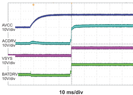
Figure 8-7. BATFET to ACFET Transition During Power Up
