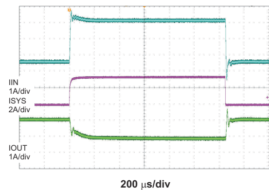
Figure 8-8. System Load Transient (Input current DPM)
