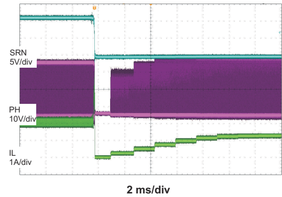
Figure 8-10. Battery to Ground Short Protection
