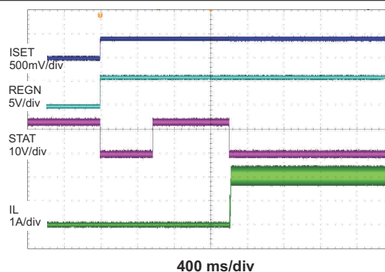
Figure 8-2. Charge Enable by ISET
