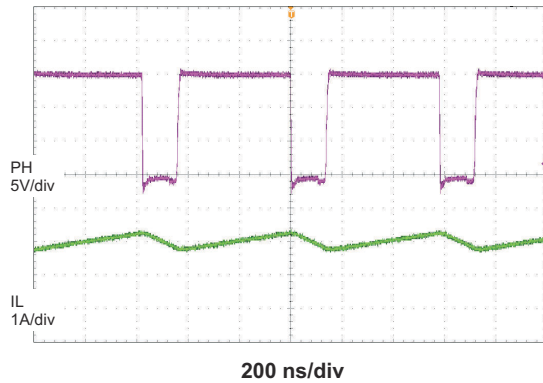
Figure 8-5. Continuous Conduction Mode Switching
