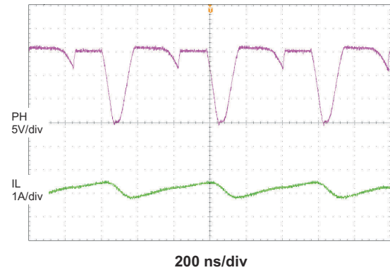
Figure 8-6. Discontinuous Conduction Mode Switching
