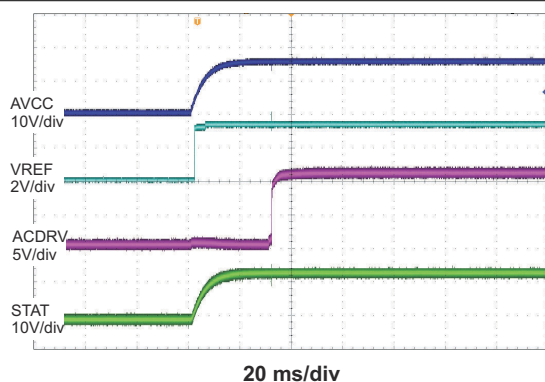
Figure 8-1. Power Up (ISET = 0)
