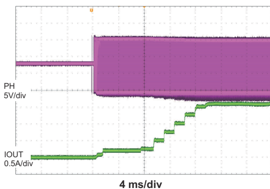
Figure 8-3. Current Soft Start
