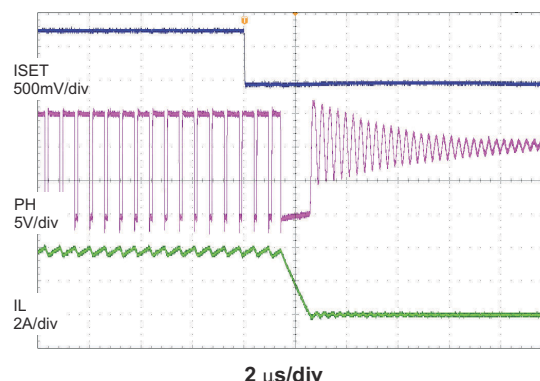
Figure 8-4. Charge Disable by ISET
