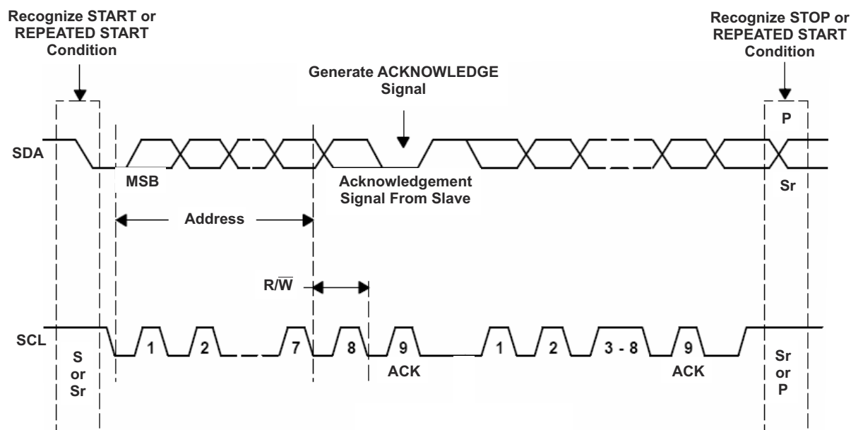
Figure 7-7. Bus Protocol
