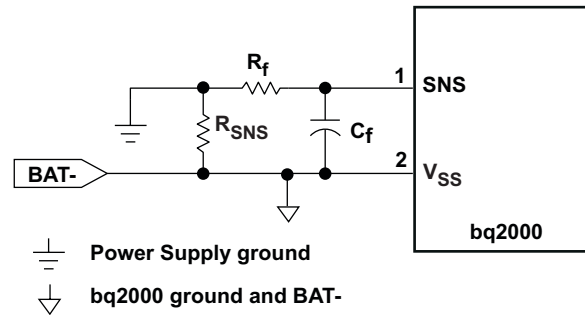
Figure 9. Current-Sensing Circuit
