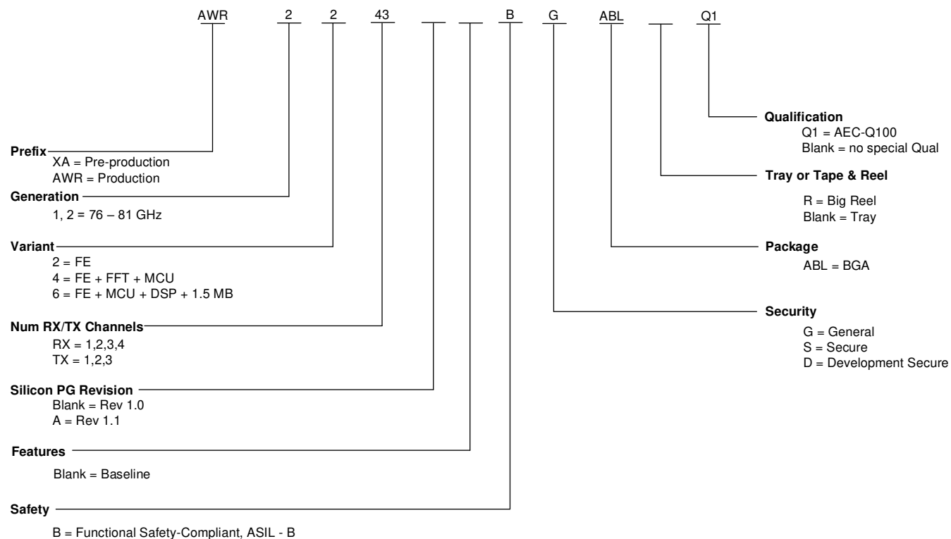
Figure 11-1. Device Nomenclature
