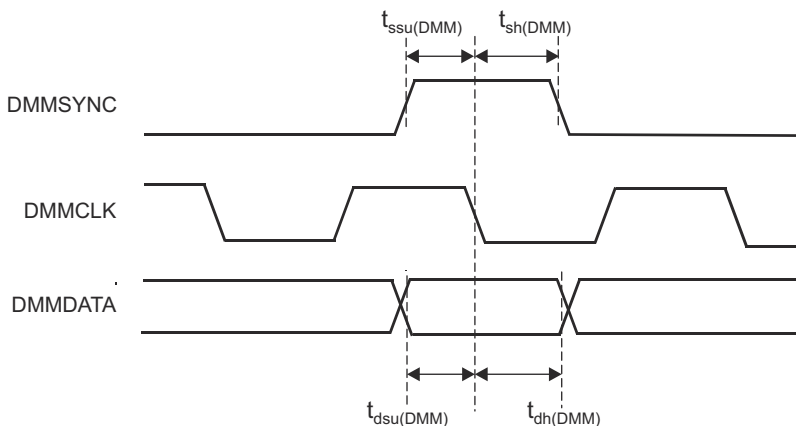
Figure 7-22. DMMDATA Timing
