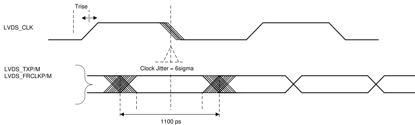
Figure 7-15. Timing Parameters
