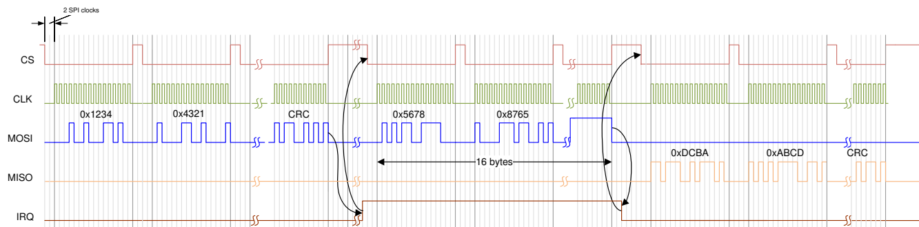
Figure 7-13. SPI Communication
