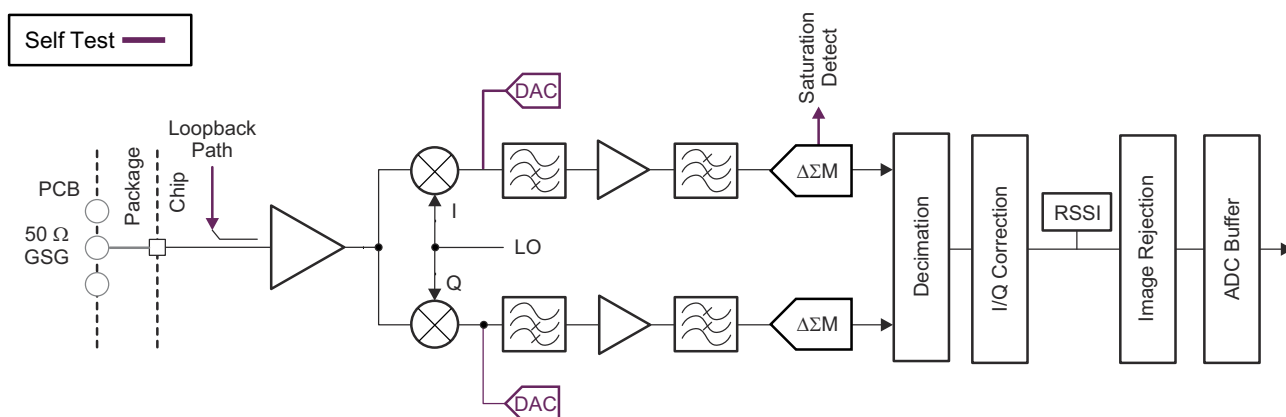
Figure 8-3. Receive Subsystem (Per Channel)
