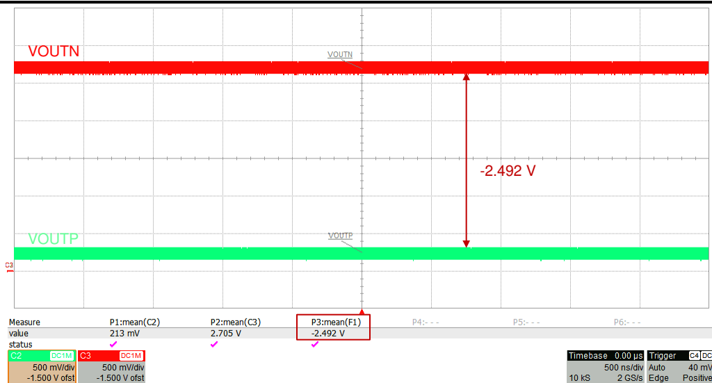
Figure 6-4. Typical Negative Clipping Output of the AMC3330
