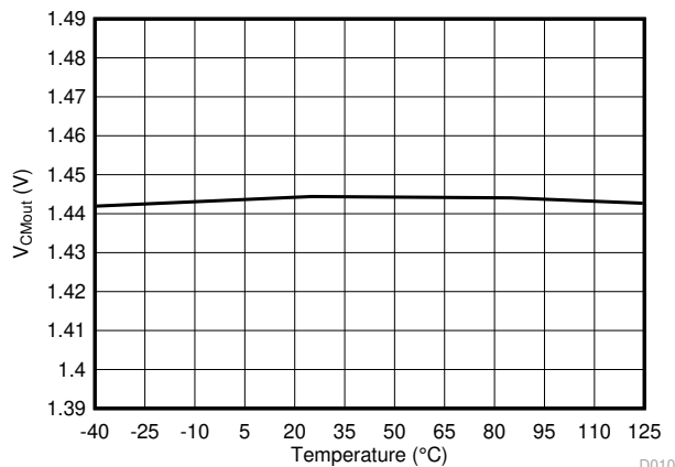
Figure 6-10. Output Common-Mode Voltage vs Temperature
