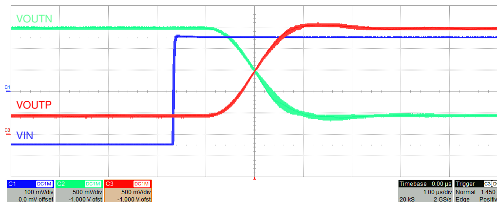
Figure 8-4. Step Response of the AMC3301-Q1
