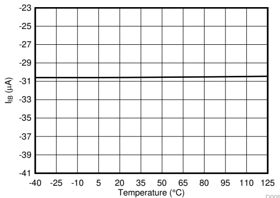
Figure 6-7. Input Bias Current vs Temperature
