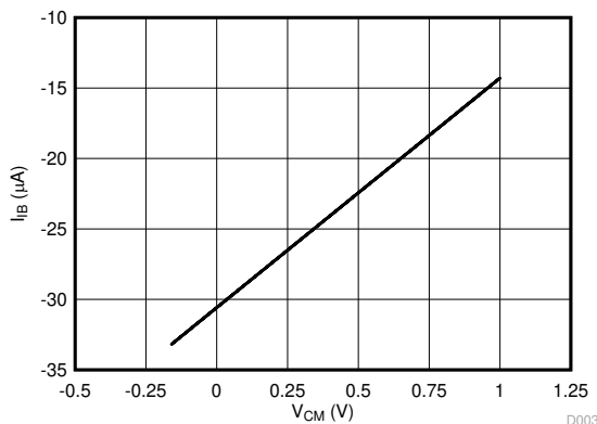
Figure 6-5. Input Bias Current vs Common-Mode Input Voltage
