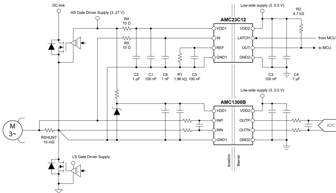
Figure 7-1. Using the AMC23C12 for Overcurrent Detection
