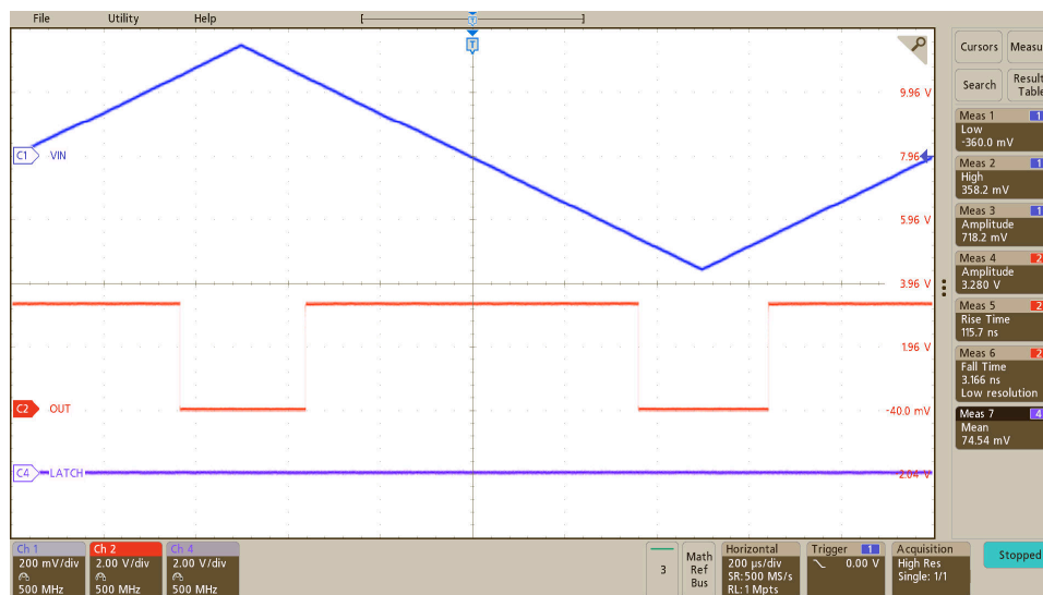
Figure 7-3. Output Response of the AMC23C12 to a Triangular Input Waveform
