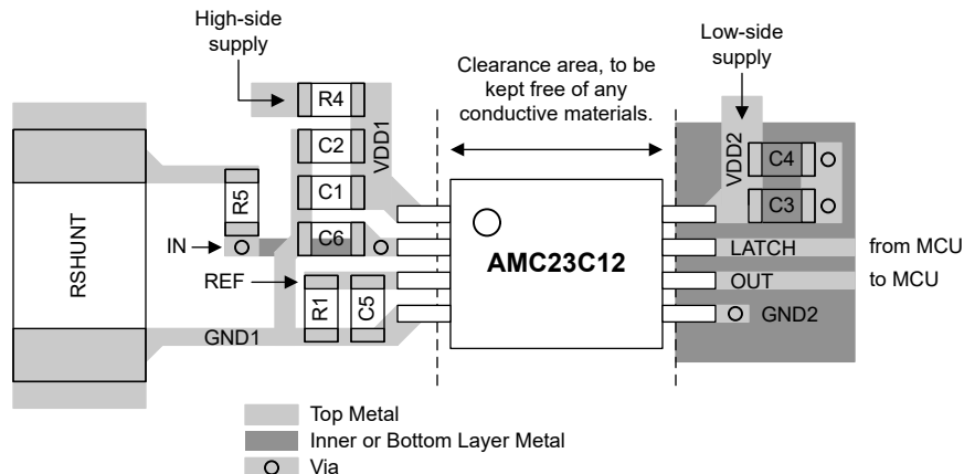
Figure 7-7. Recommended Layout of the AMC23C12
