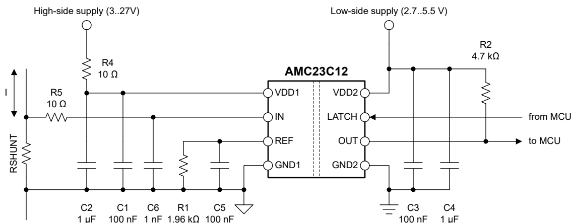
Figure 7-6. Decoupling of the AMC23C12
