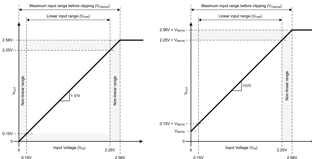
Figure 7-2. Input-to-Output Transfer Curve of the AMC0x11S Left: REFIN shorted to GND2. Right: V_{\text{REFIN}} = 150\text{mV}
