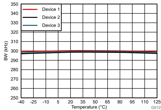
Figure 6-36. Output Bandwidth vs Temperature
