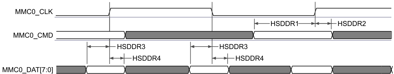
Figure 6-62. MMC0 – High Speed DDR Mode – Receive Mode
