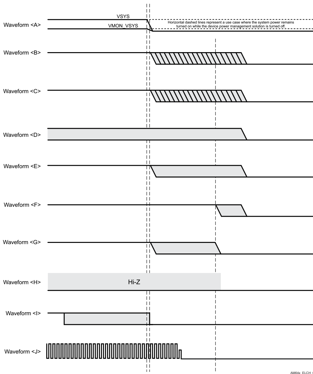
Figure 6-6. Power-Down Sequencing
