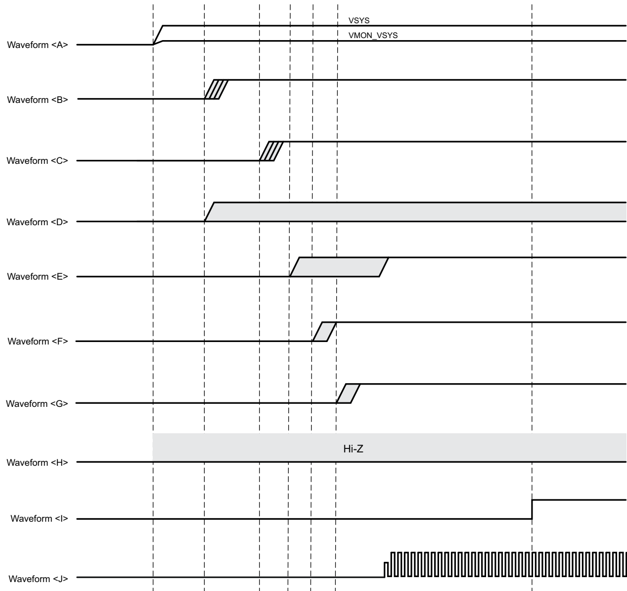
Figure 6-5. Power-Up Sequencing
