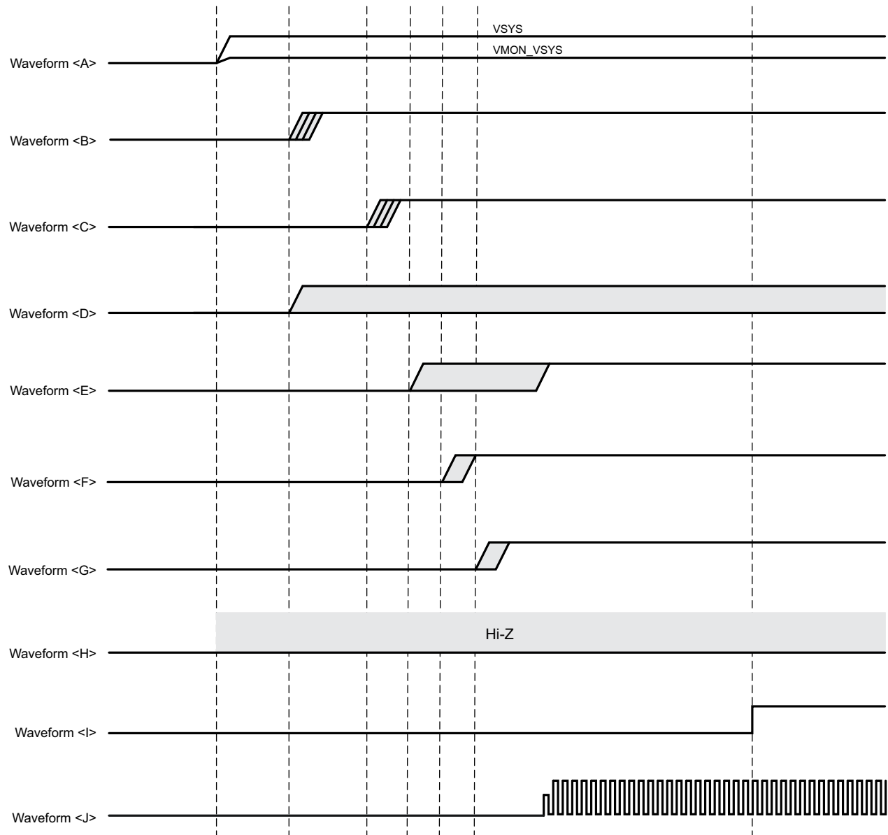
Figure 6-5. Power-Up Sequencing
