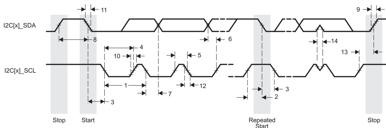
Figure 9-72. I2C Receive Timing
