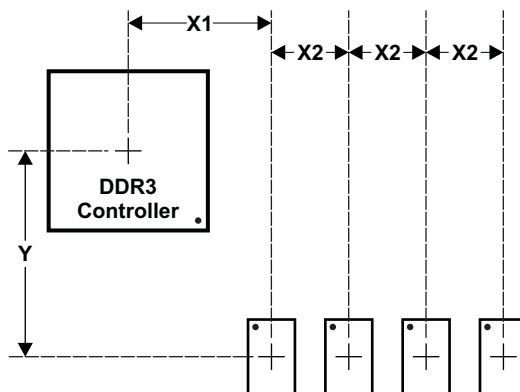
Figure 9-15. Placement Specifications
