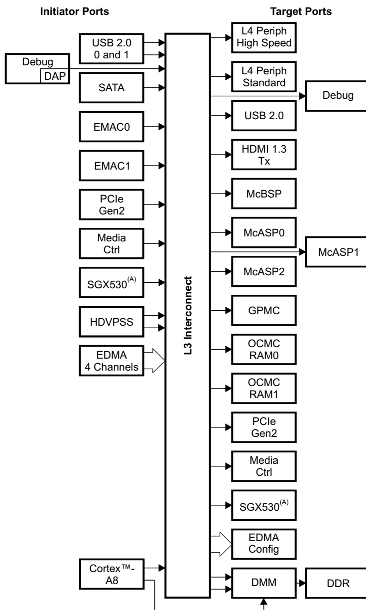
Figure 7-1. Interconnect Overview
