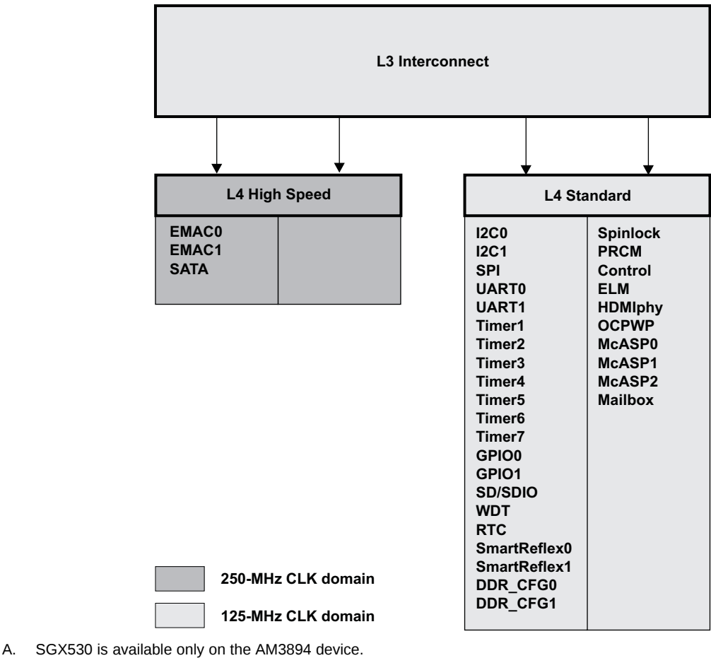
Figure 7-2. L4 Architecture
