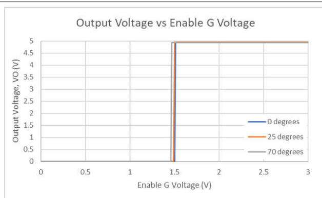
Figure 6-5. Output Voltage vs Enable G Voltage
