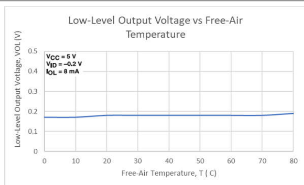
Figure 6-3. Low-Level Output Voltage vs Free-Air Temperature
