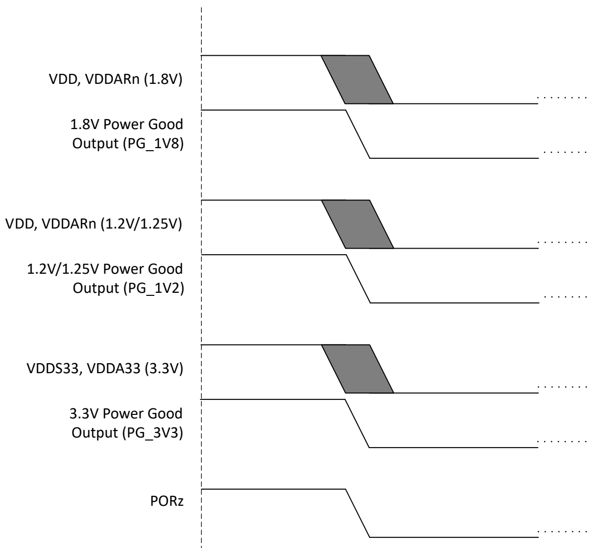
Figure 6-3. Power-Down Sequencing
