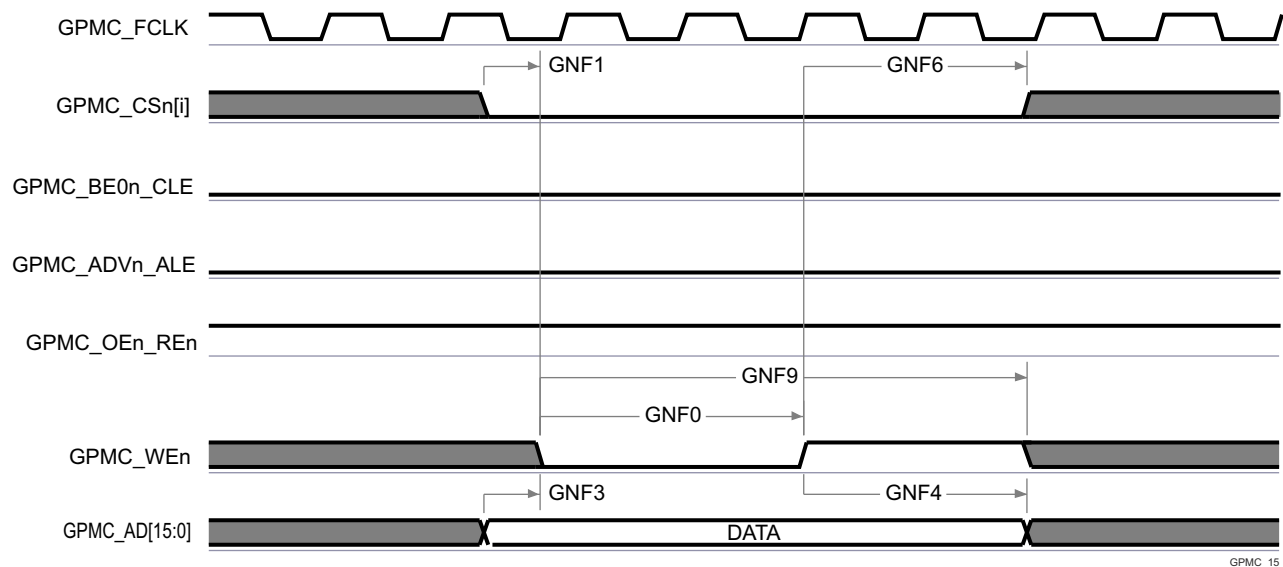
Figure 6-39. GPMC and NAND Flash — Data Read Cycle
