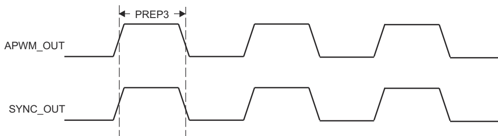
Figure 6-80. PRU-ICSS ECAP Switching Characteristics
