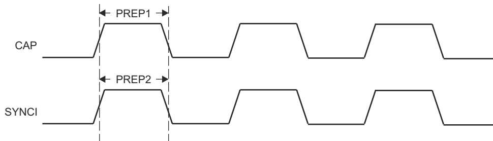
Figure 6-79. PRU-ICSS ECAP Timing
