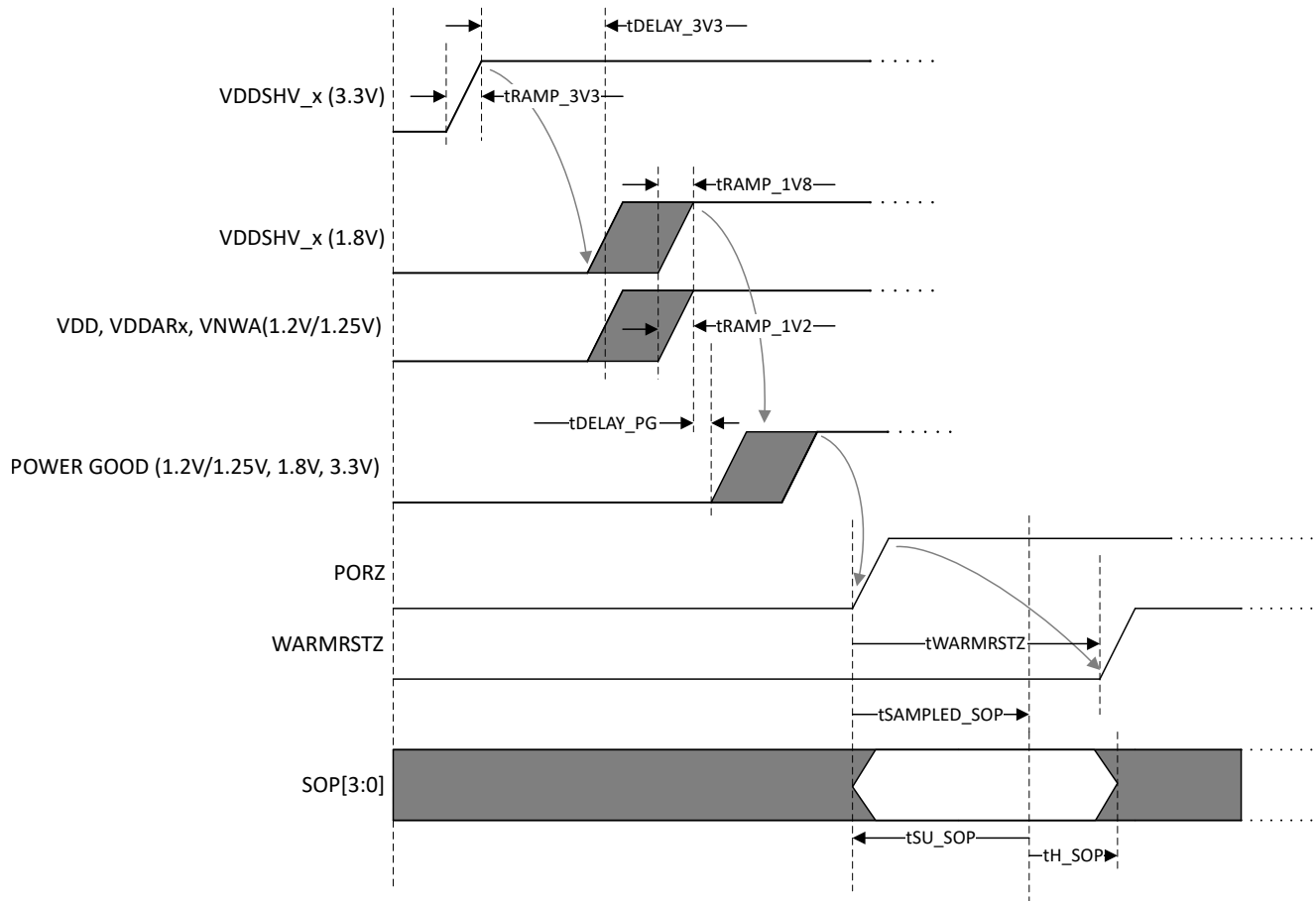
Figure 6-2. Power-On Sequencing
