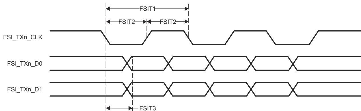
Figure 6-24. FSI Switching Characteristics - FSI Mode
