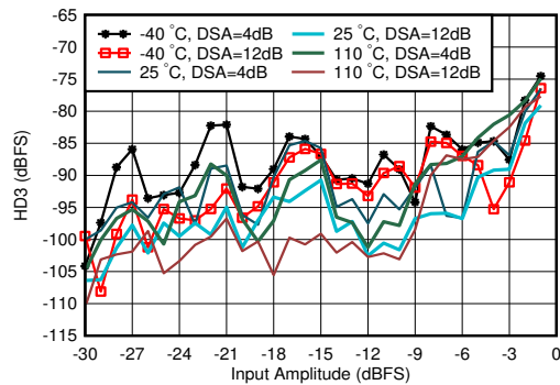
Figure 4-339. RX HD3 vs DSA Setting and Temperature at 1.9GHz
