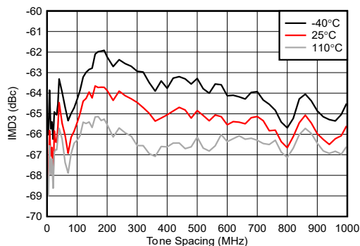
Figure 4-259. TX IMD3 vs Tone Spacing at 9.61GHz
