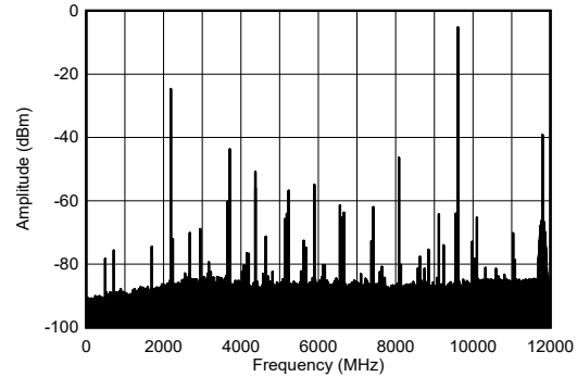
Figure 4-266. TX Single Tone Spectrum at 9.61GHz and -1dBFS (wideband)
