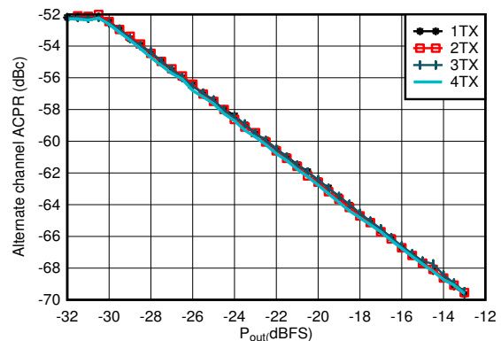
Figure 4-34. TX 20MHz LTE alt-ACPR vs Digital Level at 0.85GHz
