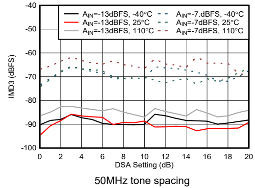
Figure 4-456. RX IMD3 vs DSA Setting at 9.6GHz
