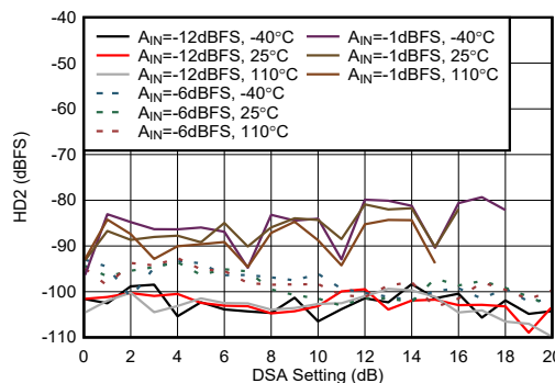
Figure 4-437. RX HD2 vs DSA Setting at 8.1GHz
