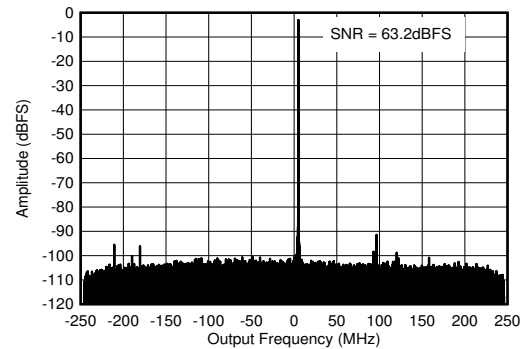
Figure 4-296. RX Output FFT at 0.8GHz
