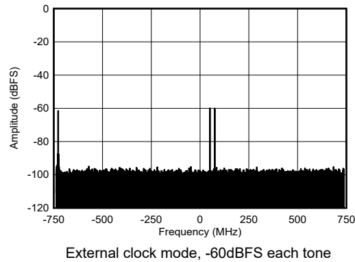
Figure 4-448. RX Dual Tone Output FFT at 8.11GHz
