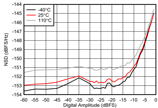
Figure 4-261. TX NSD vs Digital Amplitude at 9.61GHz
