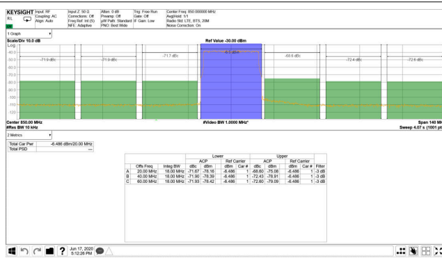
Figure 4-329. TX 20MHz LTE Output Spectrum at 0.85GHz
