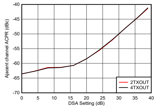
Figure 4-475. TX 20MHz LTE ACPR vs DSA Setting at 3.5GHz
