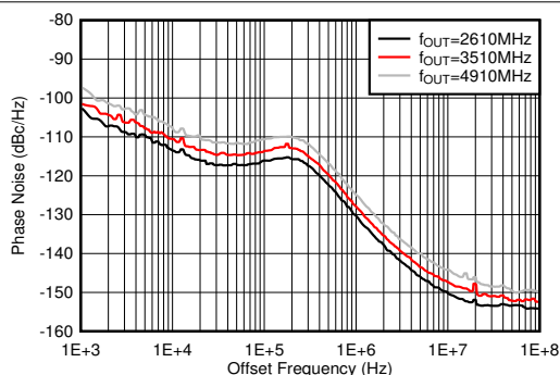
Figure 4-608. Phase Noise for 10GHz VCO vs Offset Frequency and f_{\text{OUT}} at 110^\circ\text{C}
