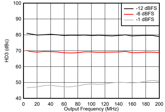
Figure 4-258. HD3 vs Frequency 0 - 200MHz
