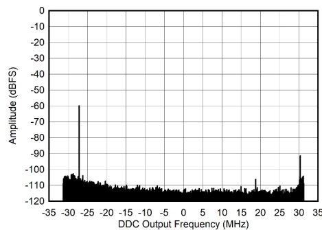
Figure 5-12. RX Output FFT at 5 MHz
