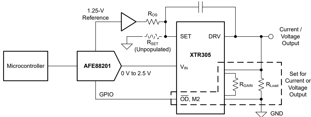
Figure 8-3. Block Diagram of the Analog Output Module Using the AFEx8201 and XTR305
