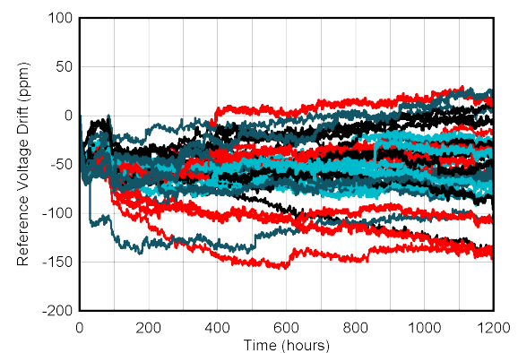
Figure 5-39. Reference Voltage Long-Term Stability
