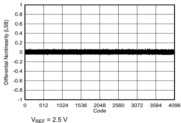
Figure 6-6. Differential Linearity Error vs Code
