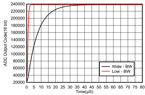
Figure 8-3. Step-Settling Performance
