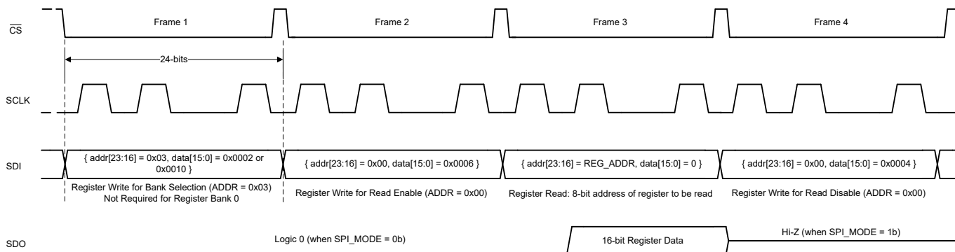
Figure 6-11. Register Read
