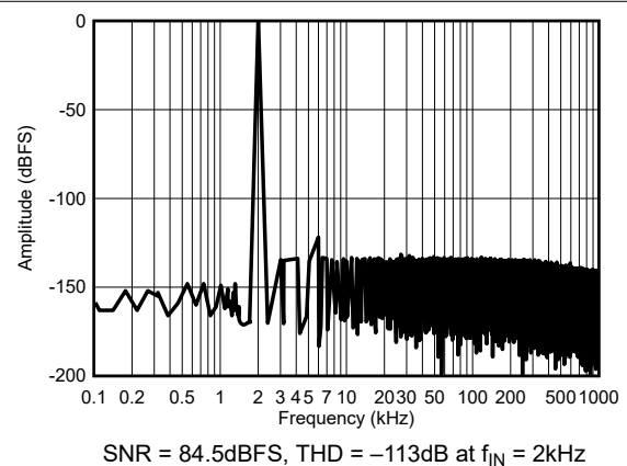
Figure 5-11. Typical FFT With Wide-Bandwidth LPF, RANGE = \pm 5V
