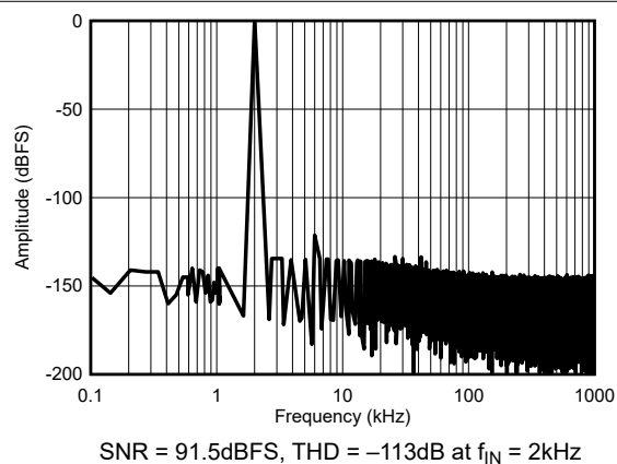
Figure 5-10. Typical FFT With Low-Bandwidth LPF, RANGE = \pm 5V
