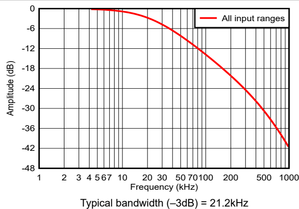
Figure 5-14. Low-Bandwidth LPF Frequency Response Across Input Ranges
