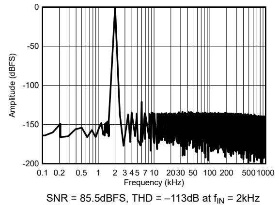
Figure 5-13. Typical FFT With Wide-Bandwidth LPF, RANGE = \pm 10V
