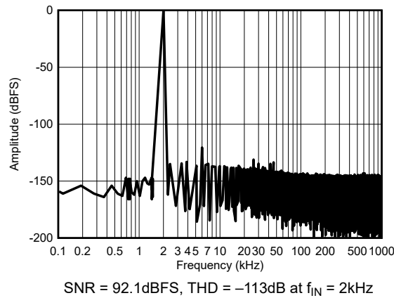
Figure 5-12. Typical FFT With Low-Bandwidth LPF, RANGE = \pm 10V
