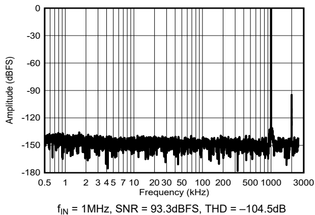
f_{IN} = 1\text{MHz} , SNR = 93.3dBFS, THD = -104.5dB Figure 6-33. Typical FFT for f_{IN} = 1\text{MHz}
