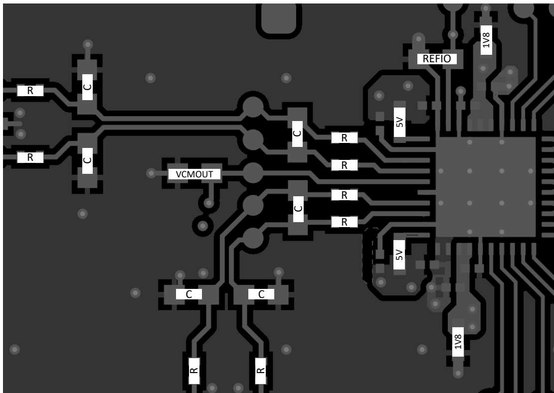
Figure 9-11. Example Layout
