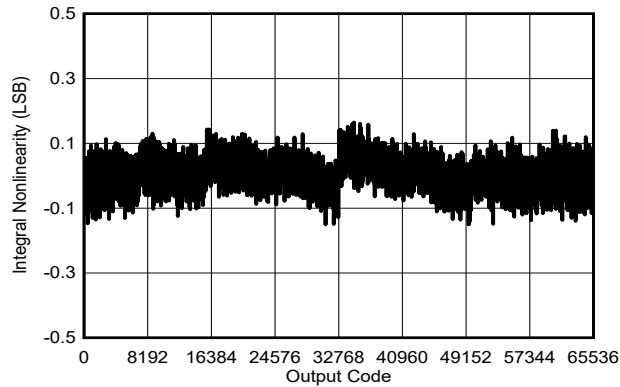
Typical INL = \pm 0.2\text{LSB} Figure 6-29. Typical INL
