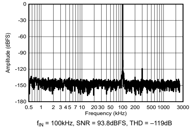
f_{IN} = 100\text{kHz} , SNR = 93.8dBFS, THD = -119dB Figure 6-32. Typical FFT for f_{IN} = 100\text{kHz}
