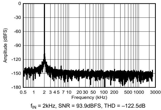
f_{IN} = 2\text{kHz} , SNR = 93.9dBFS, THD = -122.5dB Figure 6-31. Typical FFT for f_{IN} = 2\text{kHz}
